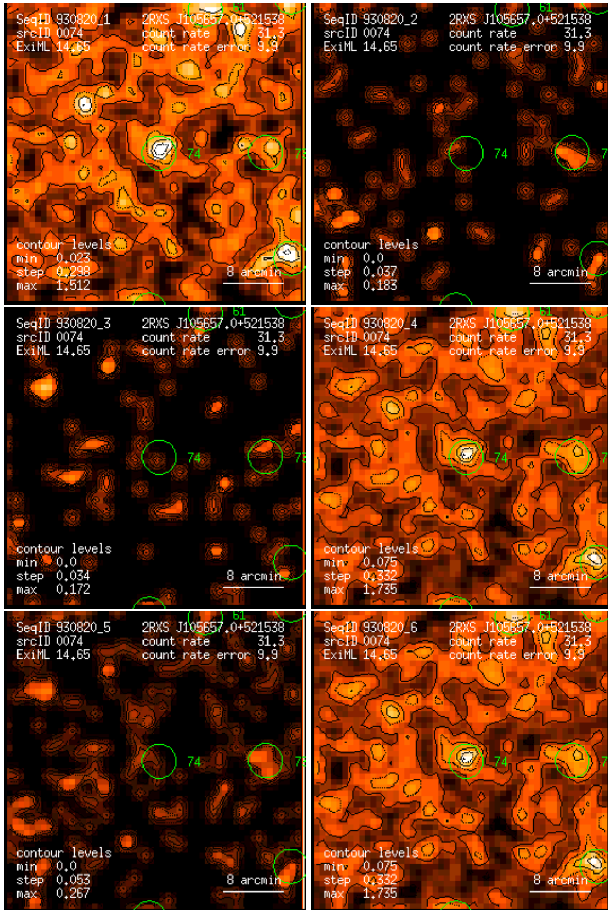
Figure 74: RASS 930820: detection 0074: band rate images, Gaussian filter: (1) PSPC channels 11 – 41, (2) 52 – 90, (3) 91 – 201, (4) 11 – 235, (5) 52 – 201, (6) 11 – 201. Broad band rates in counts/ks. Band rate contour levels in counts/ks/arcmin 2 .
