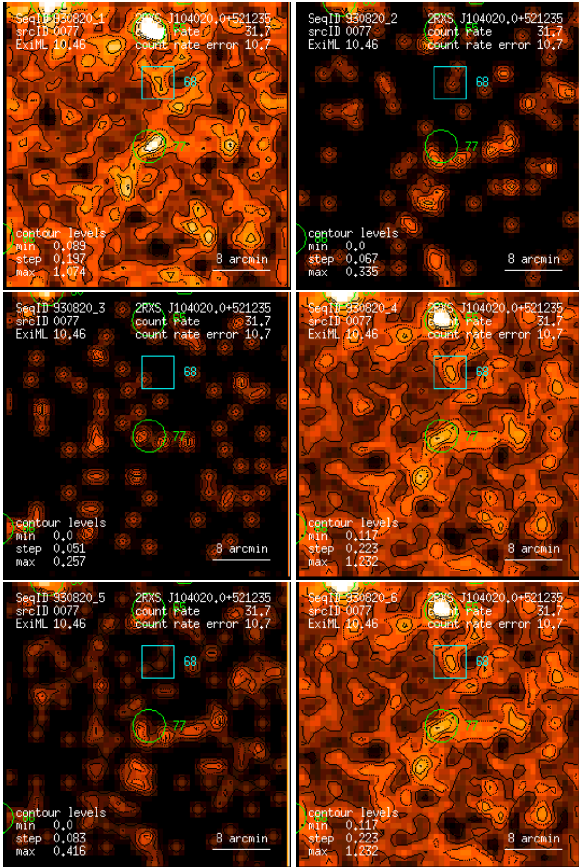
Figure 77: RASS 930820: detection 0077: band rate images, Gaussian filter: (1) PSPC channels 11 – 41, (2) 52 – 90, (3) 91 – 201, (4) 11 – 235, (5) 52 – 201, (6) 11 – 201. Broad band rates in counts/ks. Band rate contour levels in counts/ks/arcmin 2 .
