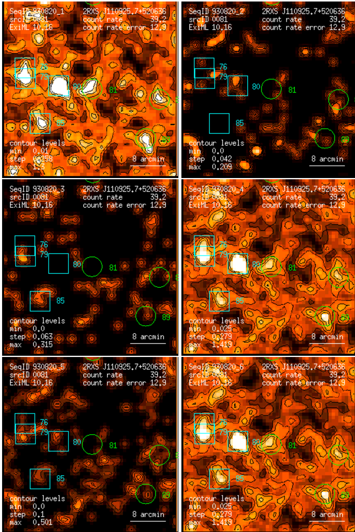
Figure 81: RASS 930820: detection 0081: band rate images, Gaussian filter: (1) PSPC channels 11 – 41, (2) 52 – 90, (3) 91 – 201, (4) 11 – 235, (5) 52 – 201, (6) 11 – 201. Broad band rates in counts/ks. Band rate contour levels in counts/ks/arcmin 2 .
