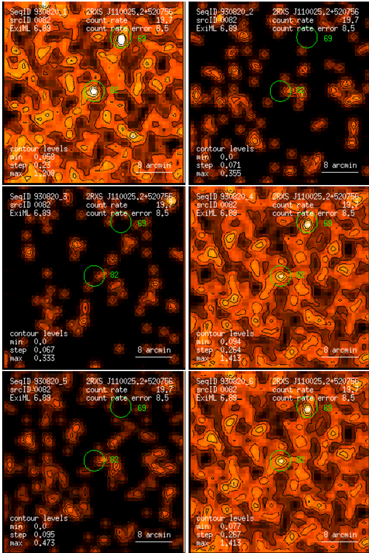
Figure 82: RASS 930820: detection 0082: band rate images, Gaussian filter: (1) PSPC channels 11 – 41, (2) 52 – 90, (3) 91 – 201, (4) 11 – 235, (5) 52 – 201, (6) 11 – 201. Broad band rates in counts/ks. Band rate contour levels in counts/ks/arcmin 2 .
