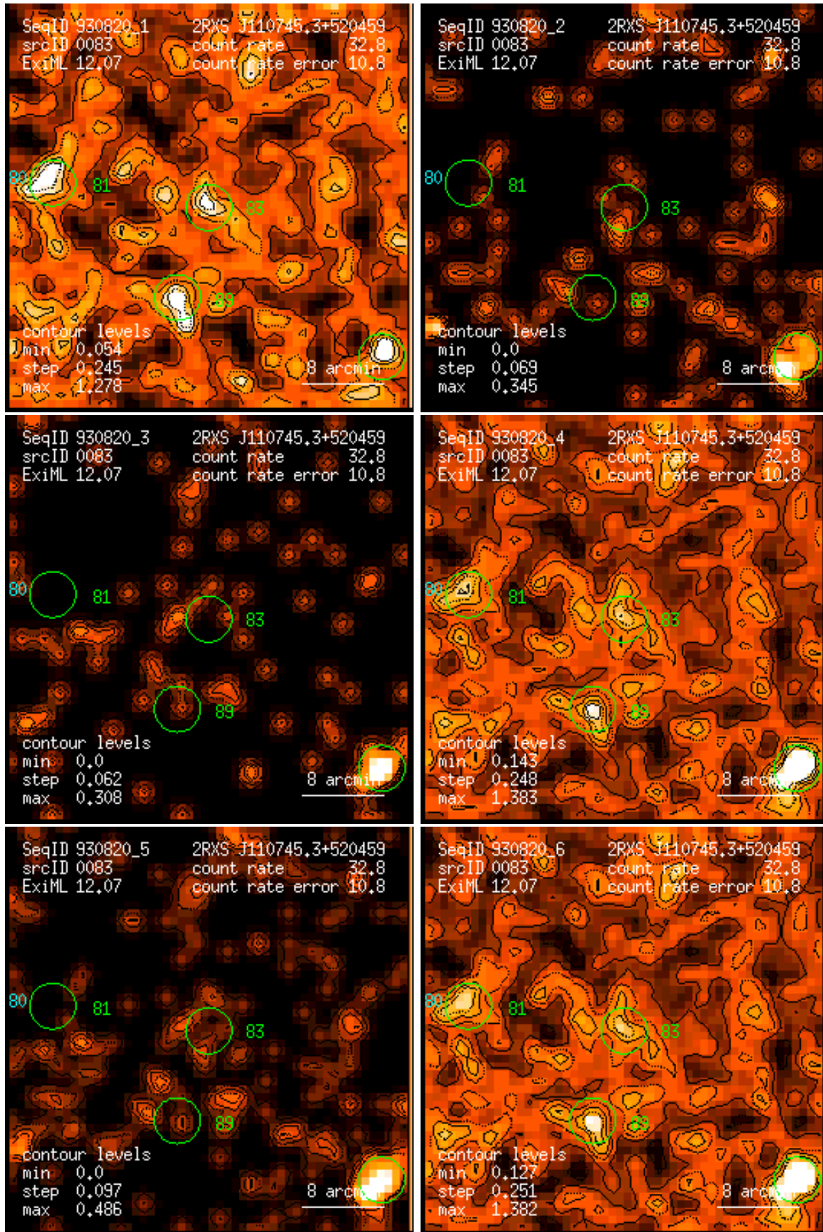
Figure 83: RASS 930820: detection 0083: band rate images, Gaussian filter: (1) PSPC channels 11 – 41, (2) 52 – 90, (3) 91 – 201, (4) 11 – 235, (5) 52 – 201, (6) 11 – 201. Broad band rates in counts/ks. Band rate contour levels in counts/ks/arcmin 2 .
