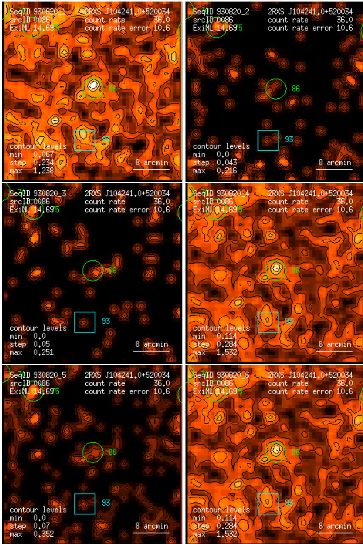
Figure 86: RASS 930820: detection 0086: band rate images, Gaussian filter: (1) PSPC channels 11 – 41, (2) 52 – 90, (3) 91 – 201, (4) 11 – 235, (5) 52 – 201, (6) 11 – 201. Broad band rates in counts/ks. Band rate contour levels in counts/ks/arcmin 2 .
