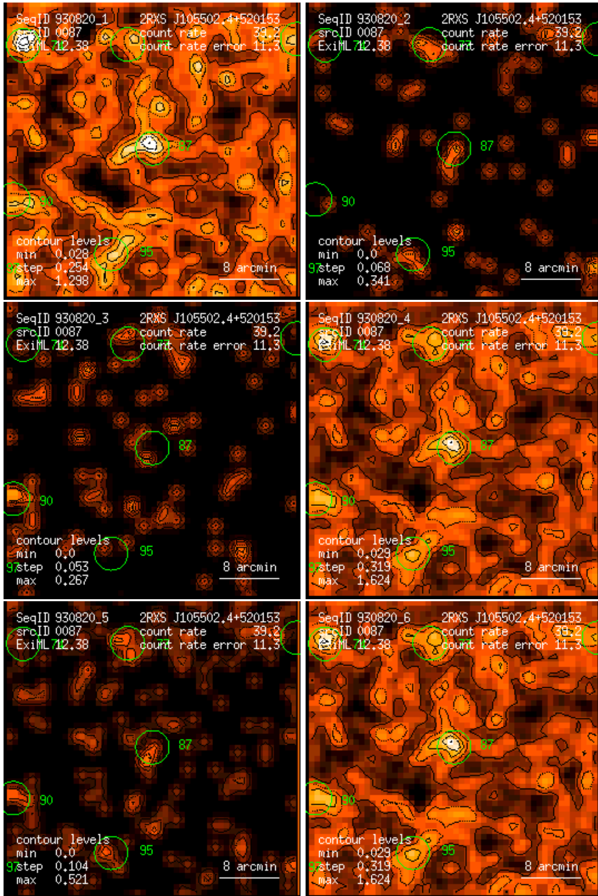
Figure 87: RASS 930820: detection 0087: band rate images, Gaussian filter: (1) PSPC channels 11 – 41, (2) 52 – 90, (3) 91 – 201, (4) 11 – 235, (5) 52 – 201, (6) 11 – 201. Broad band rates in counts/ks. Band rate contour levels in counts/ks/arcmin 2 .
