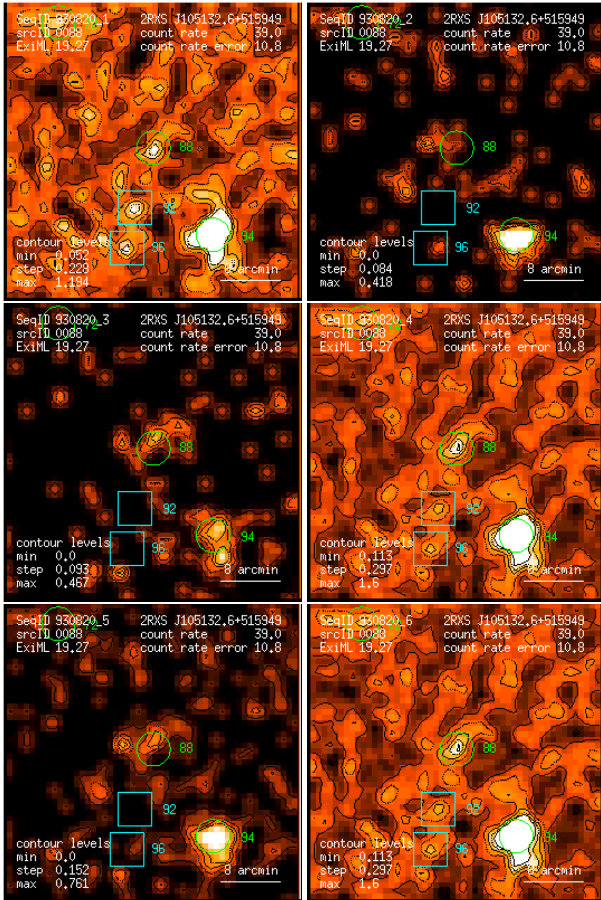
Figure 88: RASS 930820: detection 0088: band rate images, Gaussian filter: (1) PSPC channels 11 – 41, (2) 52 – 90, (3) 91 – 201, (4) 11 – 235, (5) 52 – 201, (6) 11 – 201. Broad band rates in counts/ks. Band rate contour levels in counts/ks/arcmin 2 .
