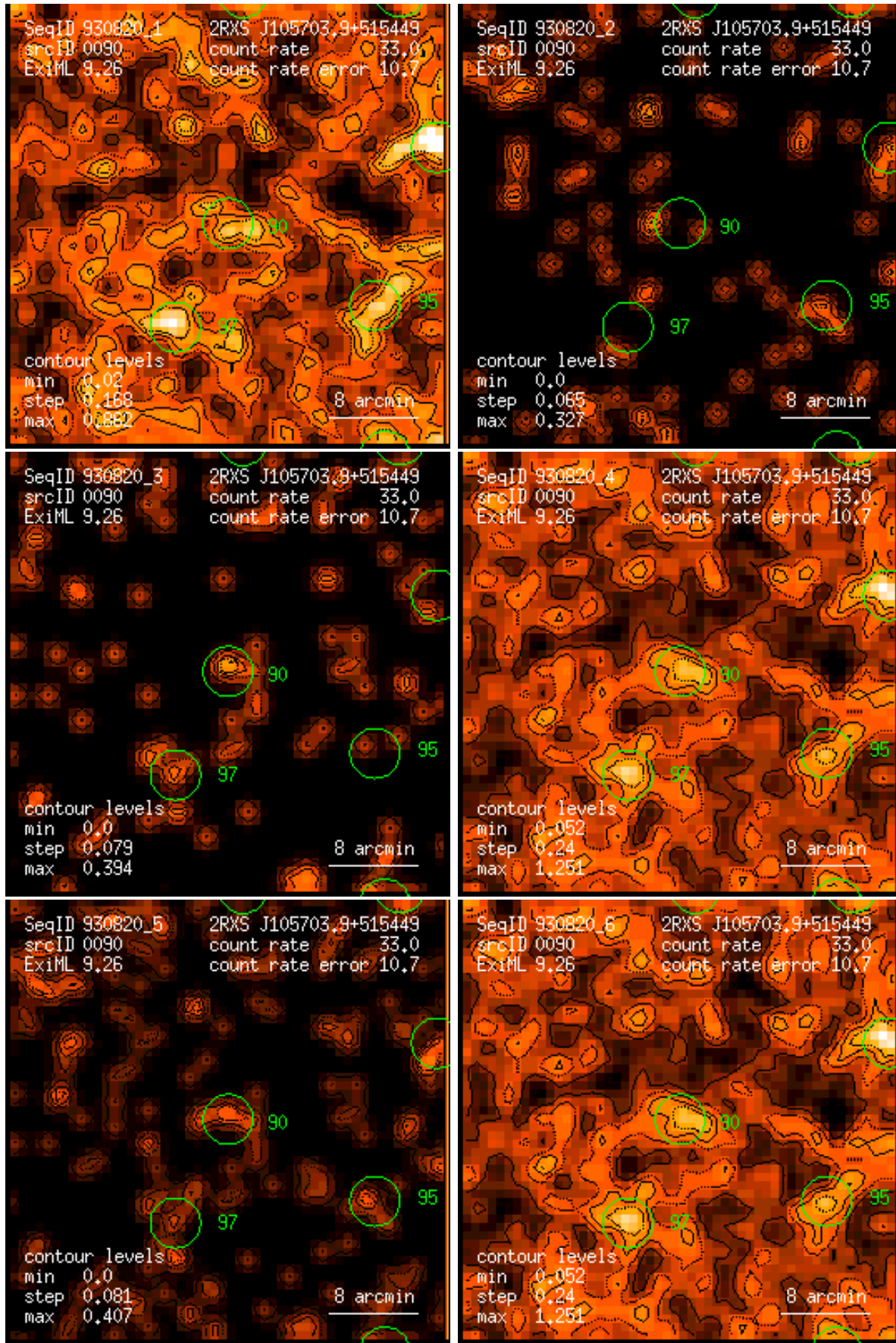
Figure 90: RASS 930820: detection 0090: band rate images, Gaussian filter: (1) PSPC channels 11 – 41, (2) 52 – 90, (3) 91 – 201, (4) 11 – 235, (5) 52 – 201, (6) 11 – 201. Broad band rates in counts/ks. Band rate contour levels in counts/ks/arcmin 2 .
