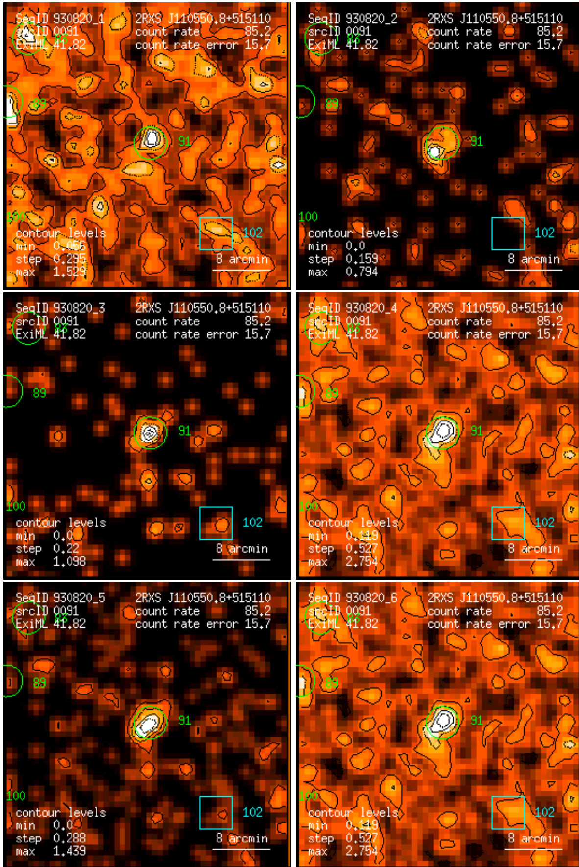
Figure 91: RASS 930820: detection 0091: band rate images, Gaussian filter: (1) PSPC channels 11 – 41, (2) 52 – 90, (3) 91 – 201, (4) 11 – 235, (5) 52 – 201, (6) 11 – 201. Broad band rates in counts/ks. Band rate contour levels in counts/ks/arcmin 2 .
