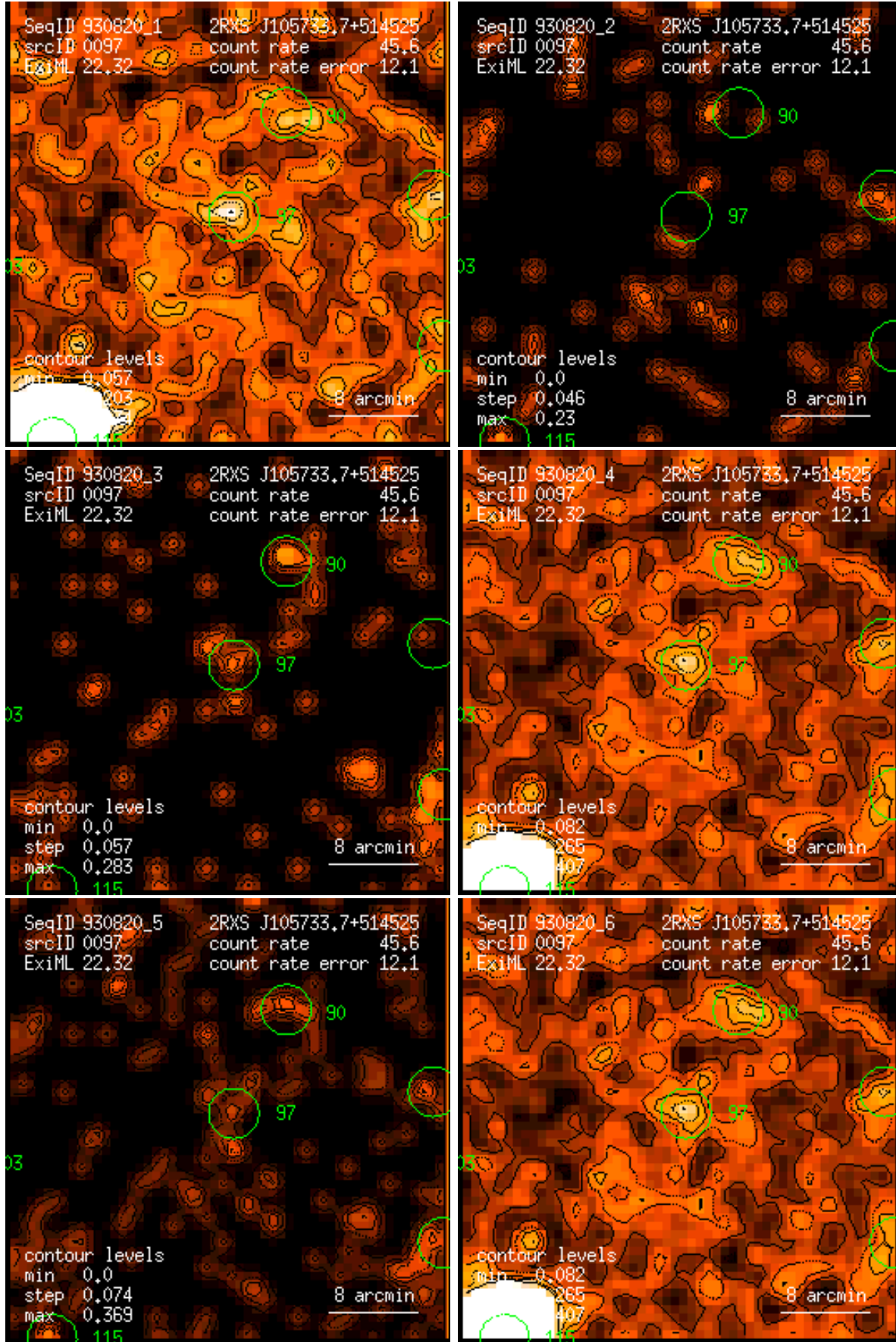
Figure 97: RASS 930820: detection 0097: band rate images, Gaussian filter: (1) PSPC channels 11 – 41, (2) 52 – 90, (3) 91 – 201, (4) 11 – 235, (5) 52 – 201, (6) 11 – 201. Broad band rates in counts/ks. Band rate contour levels in counts/ks/arcmin 2 .
