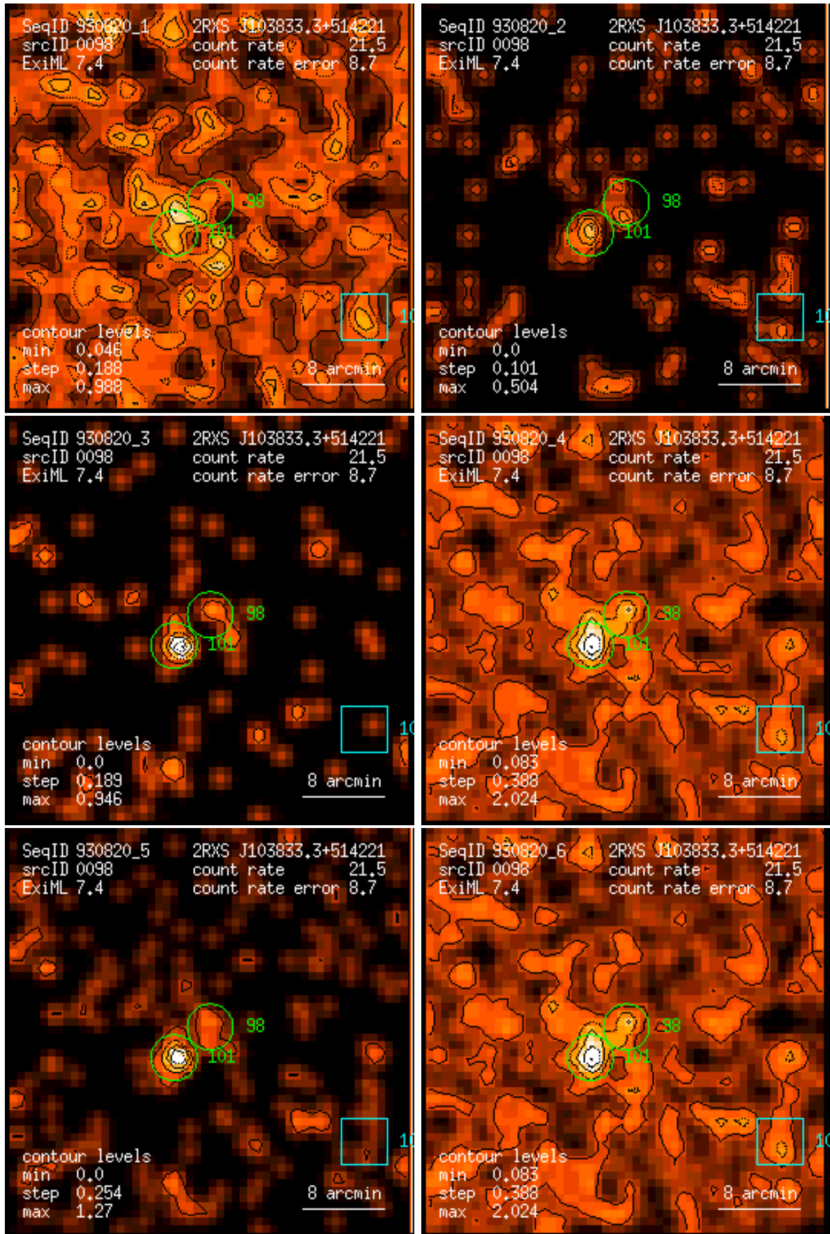
Figure 98: RASS 930820: detection 0098: band rate images, Gaussian filter: (1) PSPC channels 11 – 41, (2) 52 – 90, (3) 91 – 201, (4) 11 – 235, (5) 52 – 201, (6) 11 – 201. Broad band rates in counts/ks. Band rate contour levels in counts/ks/arcmin 2 .
