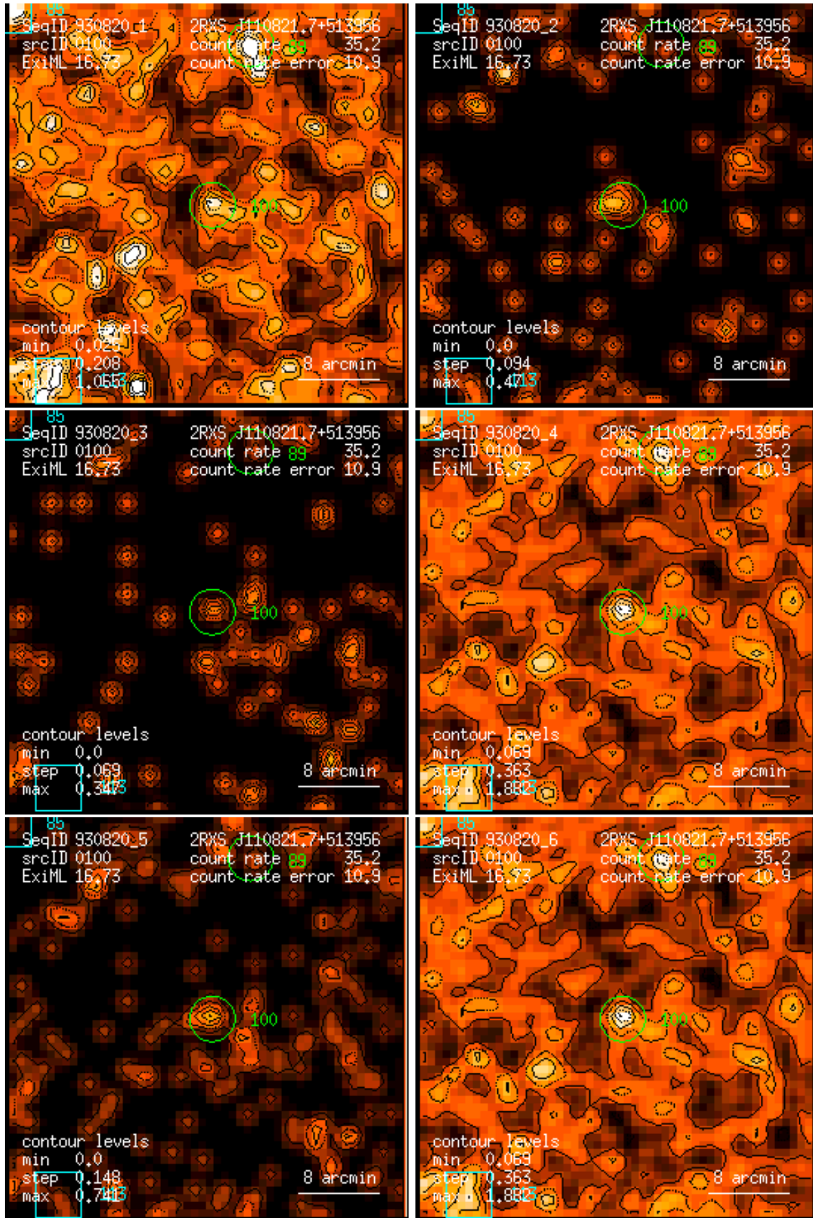
Figure 100: RASS 930820: detection 0100: band rate images, Gaussian filter: (1) PSPC channels 11 – 41, (2) 52 – 90, (3) 91 – 201, (4) 11 – 235, (5) 52 – 201, (6) 11 – 201. Broad band rates in counts/ks. Band rate contour levels in counts/ks/arcmin 2 .
