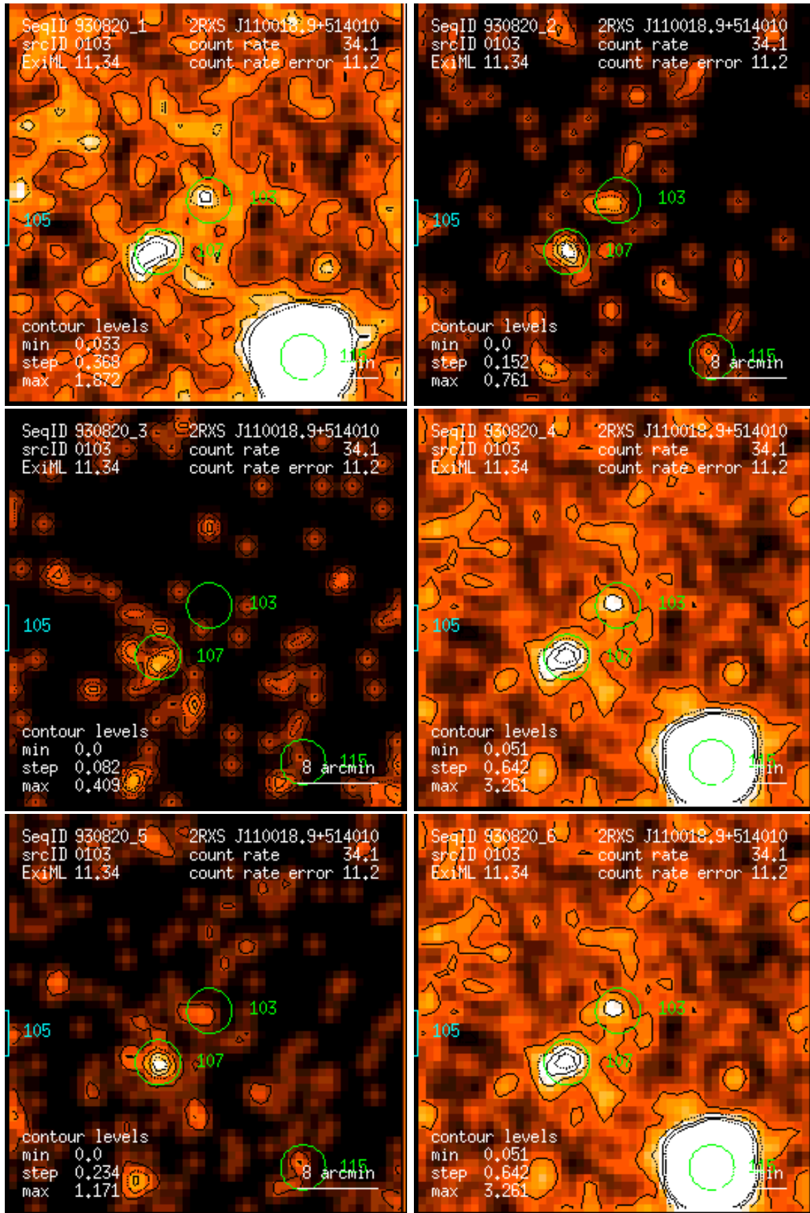
Figure 103: RASS 930820: detection 0103: band rate images, Gaussian filter: (1) PSPC channels 11 – 41, (2) 52 – 90, (3) 91 – 201, (4) 11 – 235, (5) 52 – 201, (6) 11 – 201. Broad band rates in counts/ks. Band rate contour levels in counts/ks/arcmin 2 .
