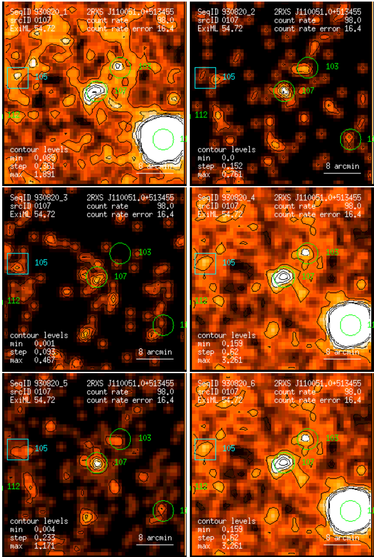
Figure 107: RASS 930820: detection 0107: band rate images, Gaussian filter: (1) PSPC channels 11 – 41, (2) 52 – 90, (3) 91 – 201, (4) 11 – 235, (5) 52 – 201, (6) 11 – 201. Broad band rates in counts/ks. Band rate contour levels in counts/ks/arcmin 2 .
