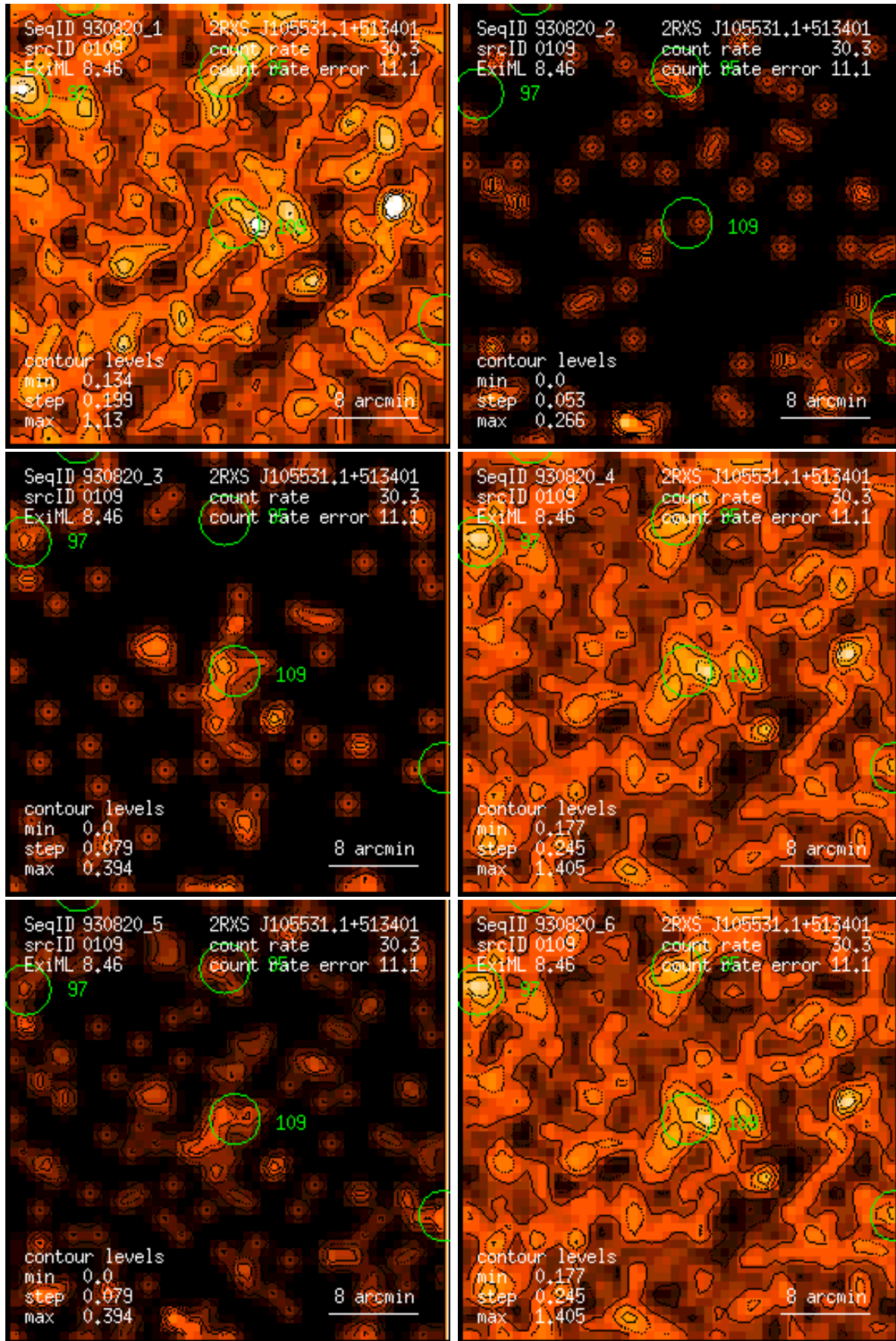
Figure 109: RASS 930820: detection 0109: band rate images, Gaussian filter: (1) PSPC channels 11 – 41, (2) 52 – 90, (3) 91 – 201, (4) 11 – 235, (5) 52 – 201, (6) 11 – 201. Broad band rates in counts/ks. Band rate contour levels in counts/ks/arcmin 2 .
