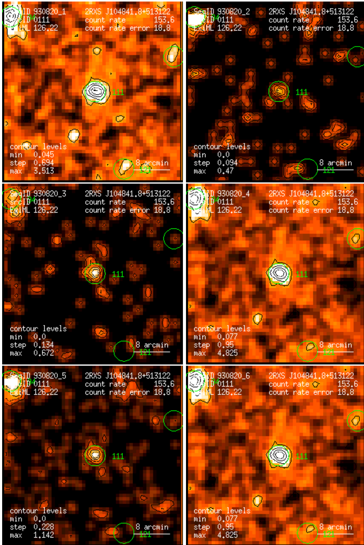
Figure 111: RASS 930820: detection 0111: band rate images, Gaussian filter: (1) PSPC channels 11 – 41, (2) 52 – 90, (3) 91 – 201, (4) 11 – 235, (5) 52 – 201, (6) 11 – 201. Broad band rates in counts/ks. Band rate contour levels in counts/ks/arcmin 2 .
