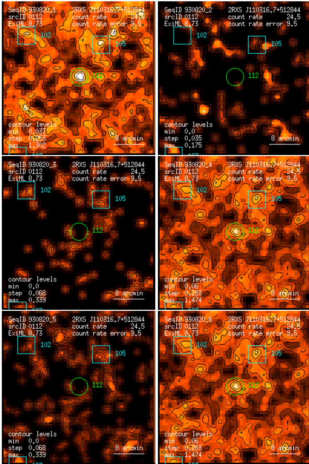
Figure 112: RASS 930820: detection 0112: band rate images, Gaussian filter: (1) PSPC channels 11 – 41, (2) 52 – 90, (3) 91 – 201, (4) 11 – 235, (5) 52 – 201, (6) 11 – 201. Broad band rates in counts/ks. Band rate contour levels in counts/ks/arcmin 2 .
