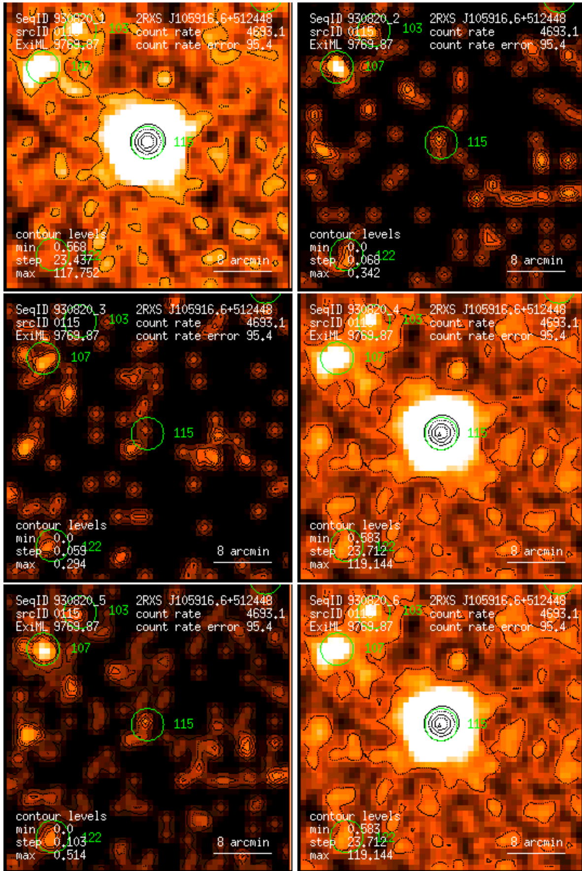
Figure 115: RASS 930820: detection 0115: band rate images, Gaussian filter: (1) PSPC channels 11 – 41, (2) 52 – 90, (3) 91 – 201, (4) 11 – 235, (5) 52 – 201, (6) 11 – 201. Broad band rates in counts/ks. Band rate contour levels in counts/ks/arcmin 2 .
