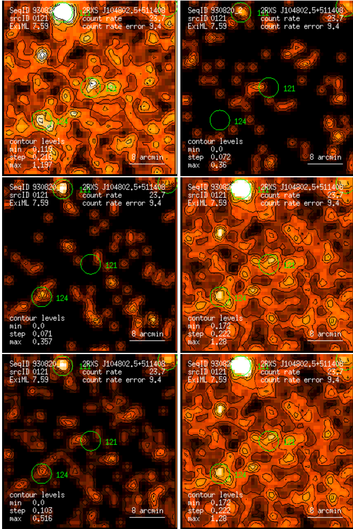
Figure 121: RASS 930820: detection 0121: band rate images, Gaussian filter: (1) PSPC channels 11 – 41, (2) 52 – 90, (3) 91 – 201, (4) 11 – 235, (5) 52 – 201, (6) 11 – 201. Broad band rates in counts/ks. Band rate contour levels in counts/ks/arcmin 2 .
