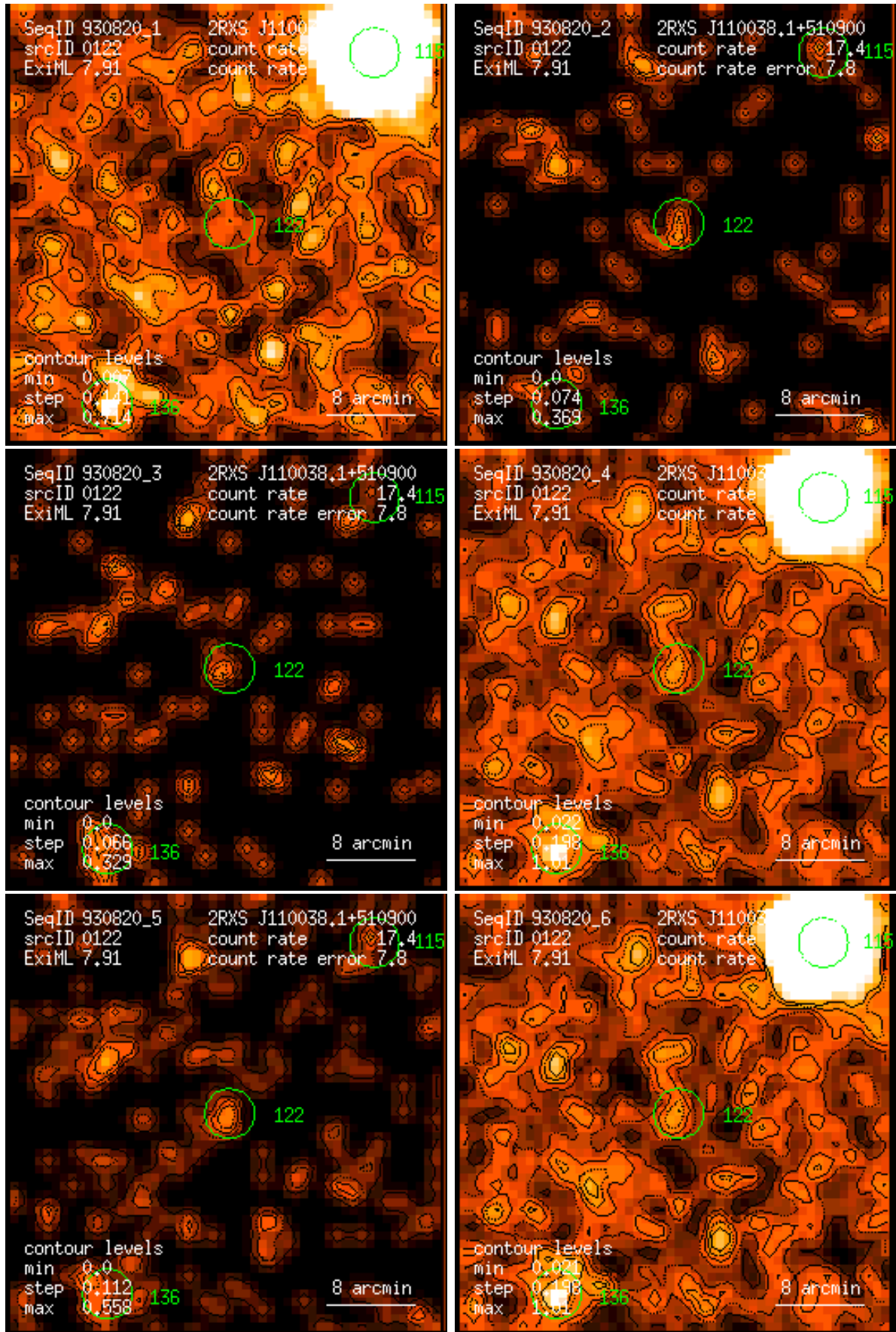
Figure 122: RASS 930820: detection 0122: band rate images, Gaussian filter: (1) PSPC channels 11 – 41, (2) 52 – 90, (3) 91 – 201, (4) 11 – 235, (5) 52 – 201, (6) 11 – 201. Broad band rates in counts/ks. Band rate contour levels in counts/ks/arcmin 2 .
