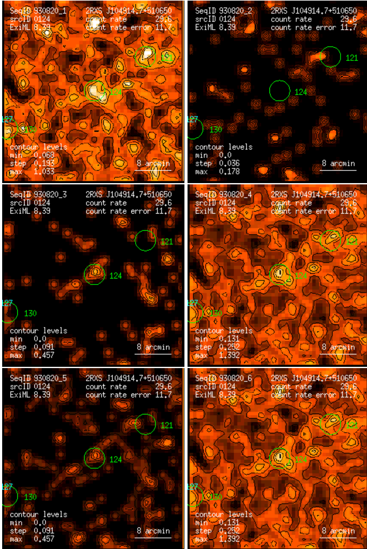
Figure 124: RASS 930820: detection 0124: band rate images, Gaussian filter: (1) PSPC channels 11 – 41, (2) 52 – 90, (3) 91 – 201, (4) 11 – 235, (5) 52 – 201, (6) 11 – 201. Broad band rates in counts/ks. Band rate contour levels in counts/ks/arcmin 2 .
