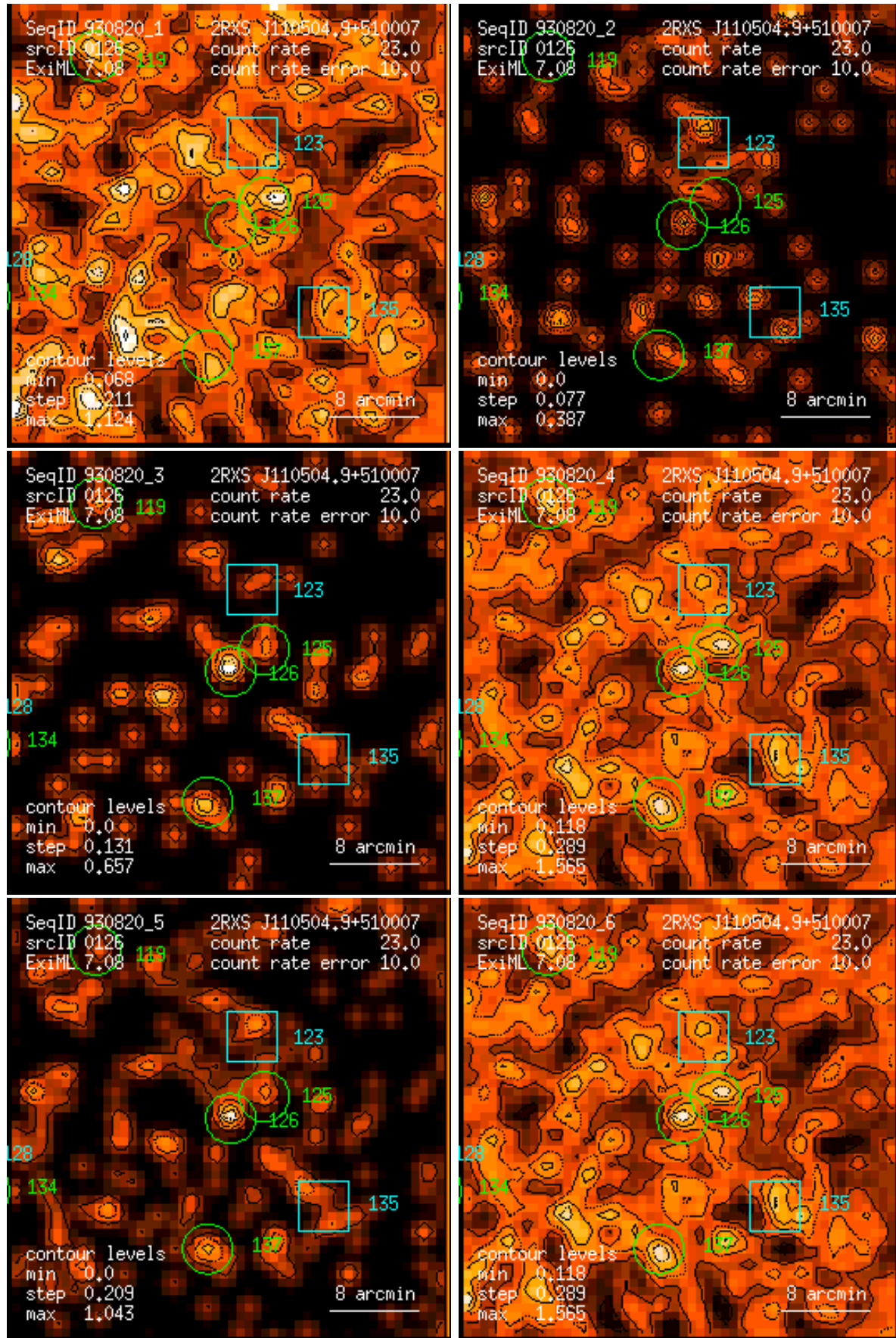
Figure 126: RASS 930820: detection 0126: band rate images, Gaussian filter: (1) PSPC channels 11 – 41, (2) 52 – 90, (3) 91 – 201, (4) 11 – 235, (5) 52 – 201, (6) 11 – 201. Broad band rates in counts/ks. Band rate contour levels in counts/ks/arcmin 2 .
