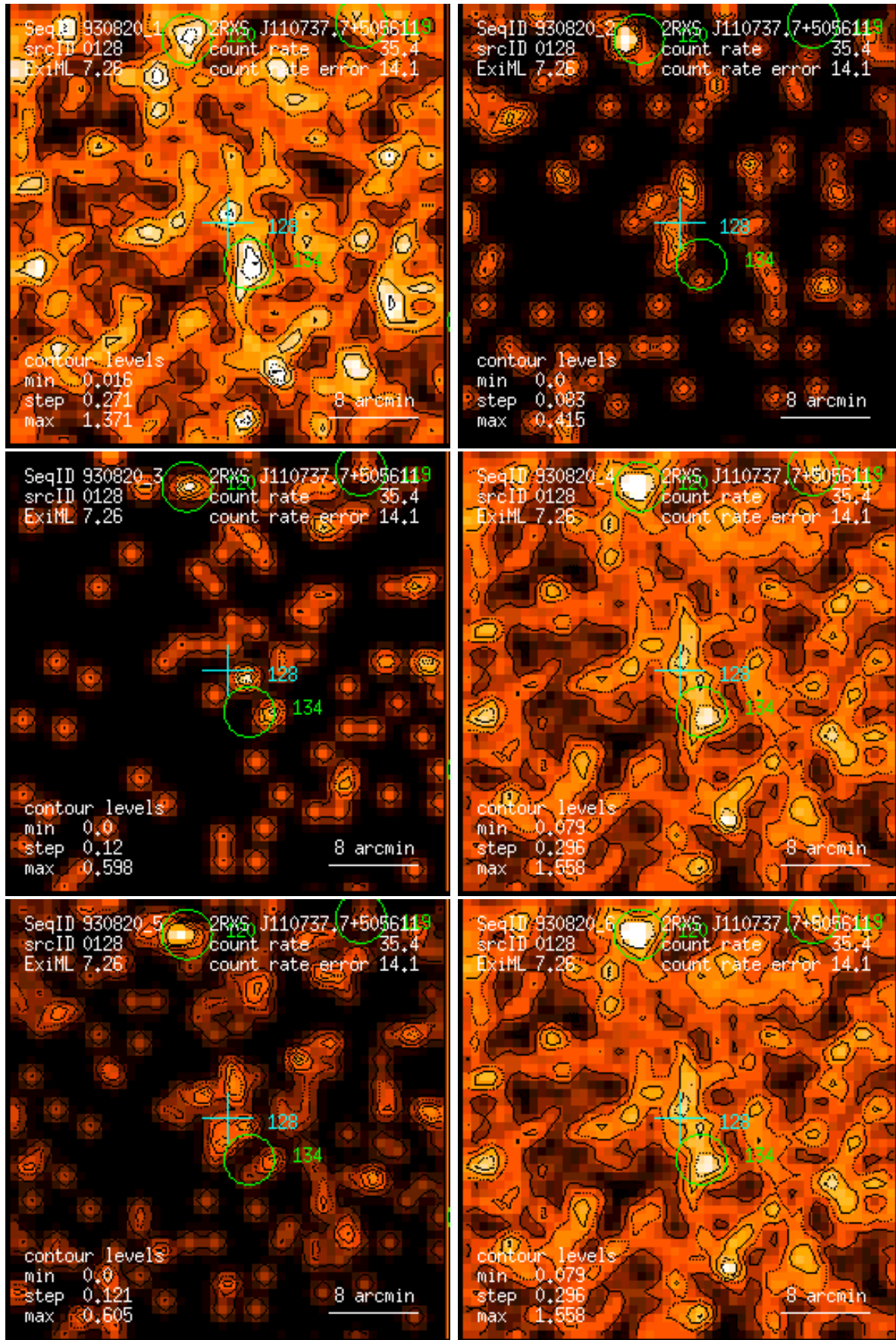
Figure 128: RASS 930820: detection 0128: band rate images, Gaussian filter: (1) PSPC channels 11 – 41, (2) 52 – 90, (3) 91 – 201, (4) 11 – 235, (5) 52 – 201, (6) 11 – 201. Broad band rates in counts/ks. Band rate contour levels in counts/ks/arcmin 2 .
