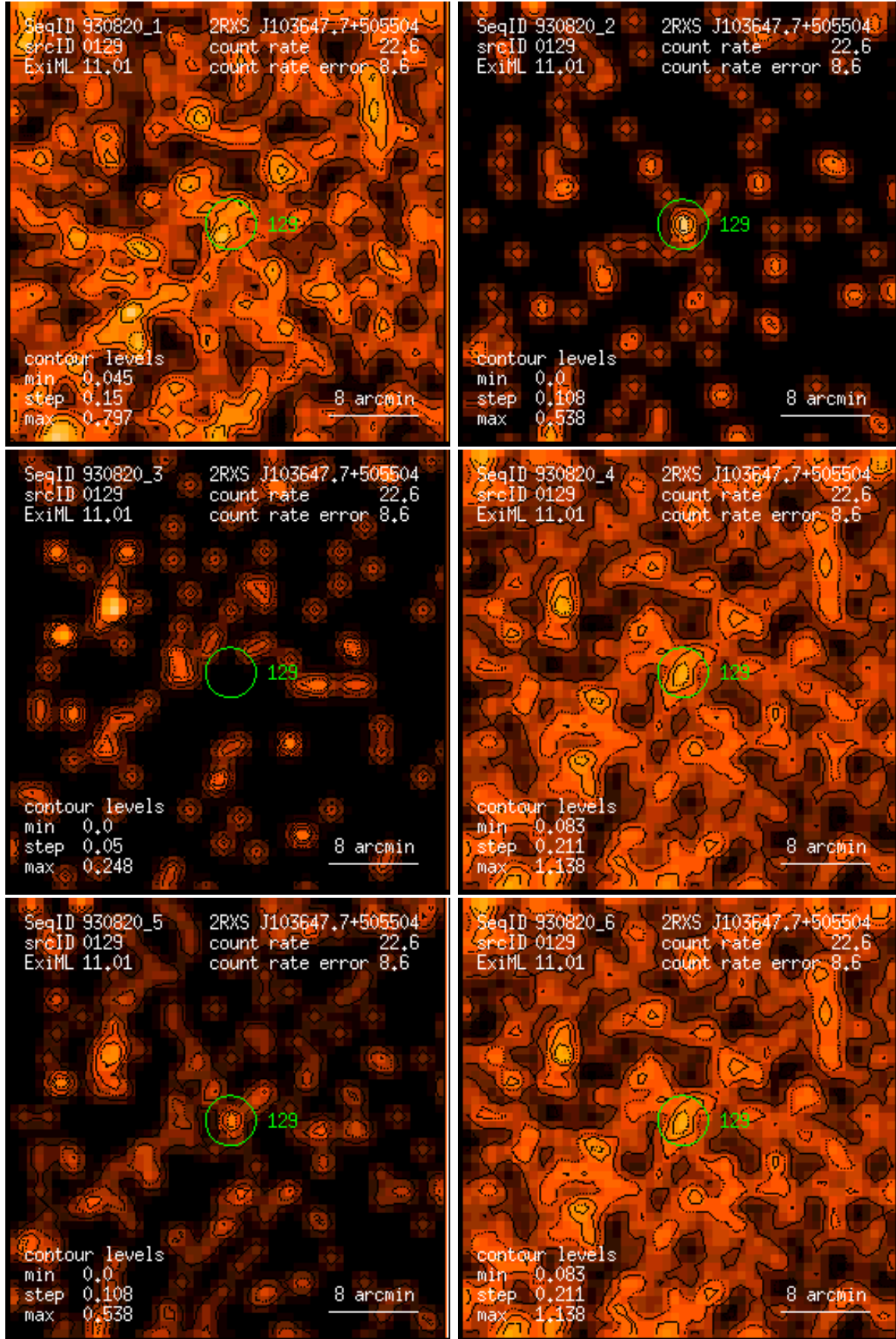
Figure 129: RASS 930820: detection 0129: band rate images, Gaussian filter: (1) PSPC channels 11 – 41, (2) 52 – 90, (3) 91 – 201, (4) 11 – 235, (5) 52 – 201, (6) 11 – 201. Broad band rates in counts/ks. Band rate contour levels in counts/ks/arcmin 2 .
