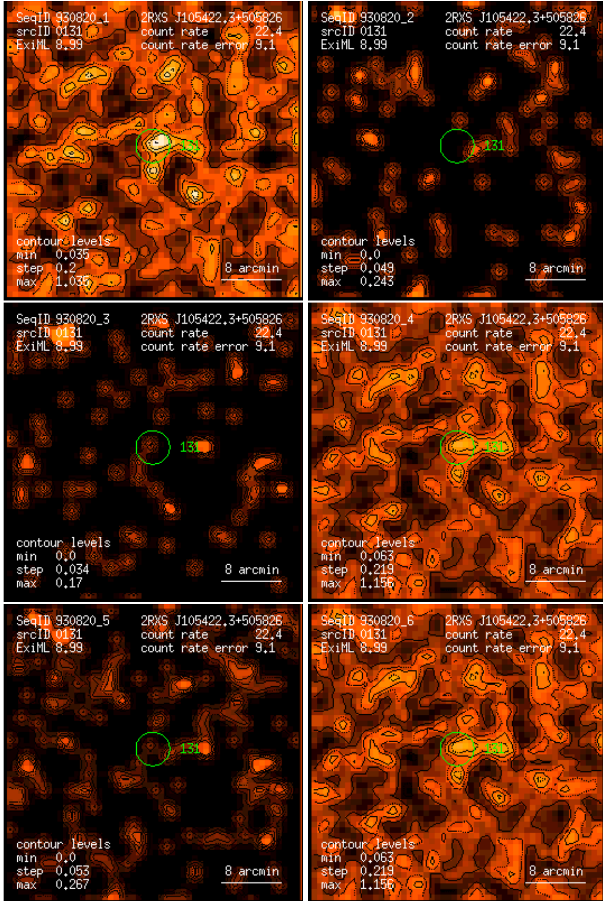
Figure 131: RASS 930820: detection 0131: band rate images, Gaussian filter: (1) PSPC channels 11 – 41, (2) 52 – 90, (3) 91 – 201, (4) 11 – 235, (5) 52 – 201, (6) 11 – 201. Broad band rates in counts/ks. Band rate contour levels in counts/ks/arcmin 2 .
