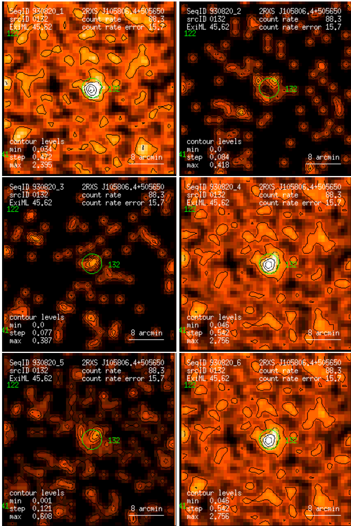
Figure 132: RASS 930820: detection 0132: band rate images, Gaussian filter: (1) PSPC channels 11 – 41, (2) 52 – 90, (3) 91 – 201, (4) 11 – 235, (5) 52 – 201, (6) 11 – 201. Broad band rates in counts/ks. Band rate contour levels in counts/ks/arcmin 2 .
