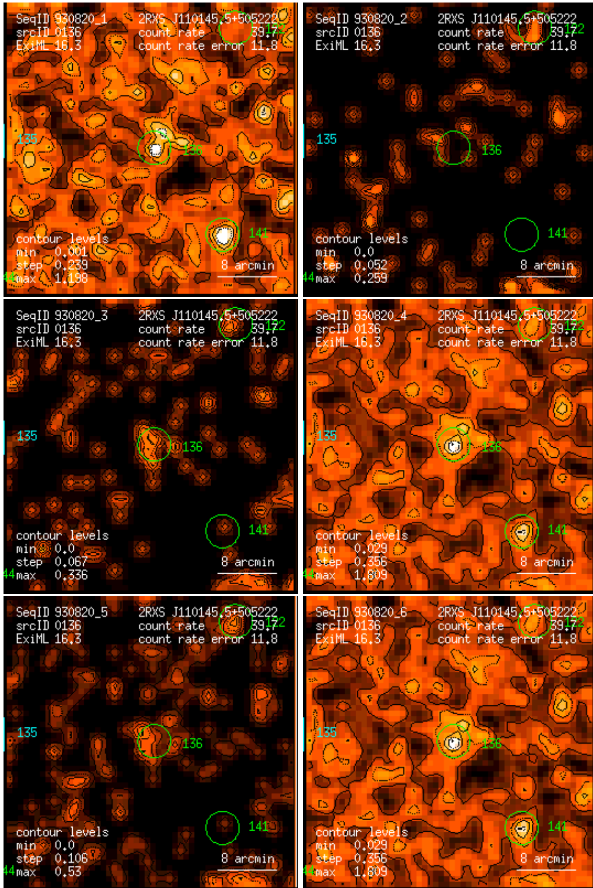
Figure 136: RASS 930820: detection 0136: band rate images, Gaussian filter: (1) PSPC channels 11 – 41, (2) 52 – 90, (3) 91 – 201, (4) 11 – 235, (5) 52 – 201, (6) 11 – 201. Broad band rates in counts/ks. Band rate contour levels in counts/ks/arcmin 2 .
