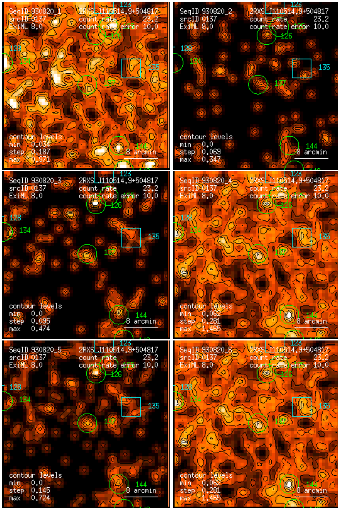
Figure 137: RASS 930820: detection 0137: band rate images, Gaussian filter: (1) PSPC channels 11 – 41, (2) 52 – 90, (3) 91 – 201, (4) 11 – 235, (5) 52 – 201, (6) 11 – 201. Broad band rates in counts/ks. Band rate contour levels in counts/ks/arcmin 2 .
