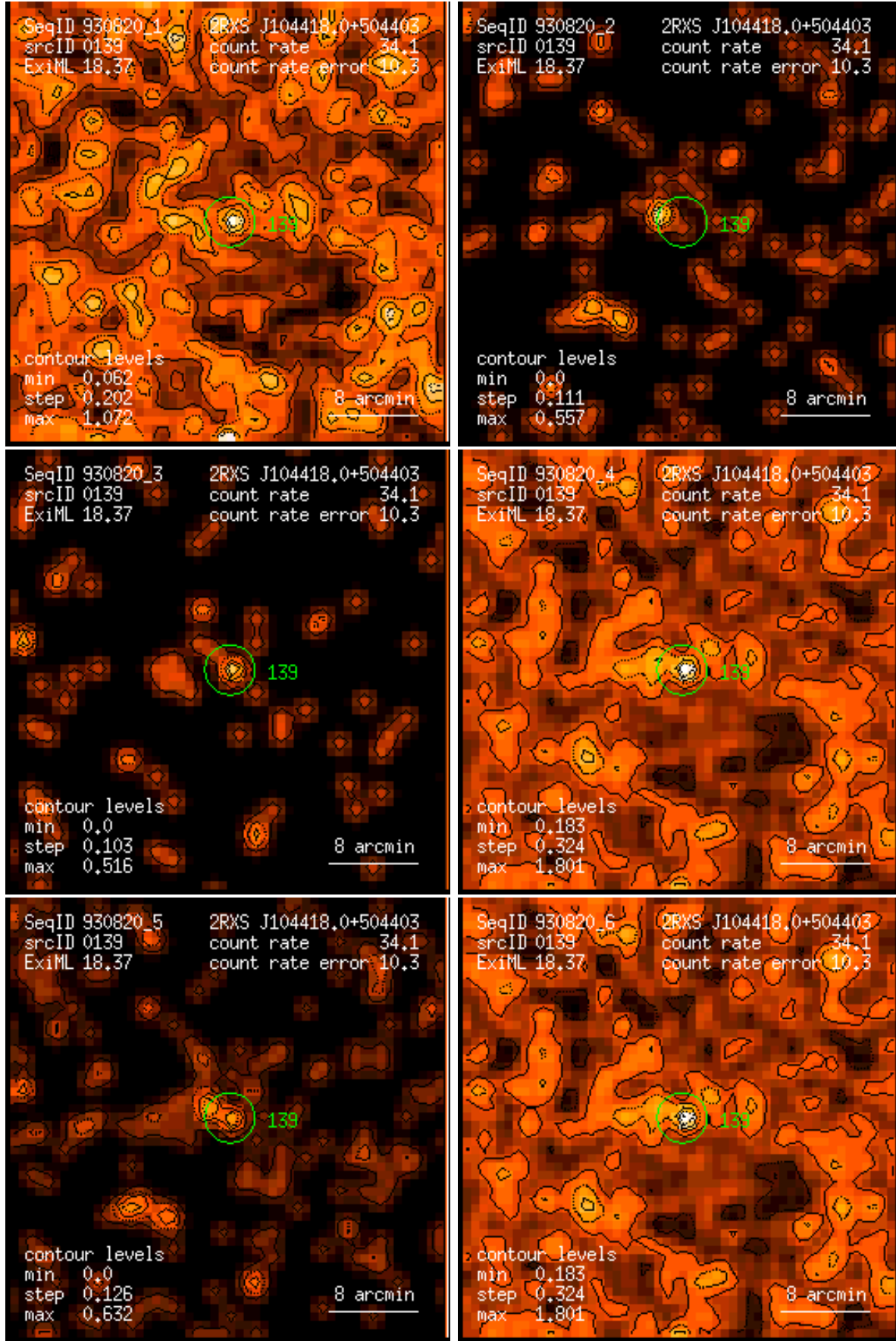
Figure 139: RASS 930820: detection 0139: band rate images, Gaussian filter: (1) PSPC channels 11 – 41, (2) 52 – 90, (3) 91 – 201, (4) 11 – 235, (5) 52 – 201, (6) 11 – 201. Broad band rates in counts/ks. Band rate contour levels in counts/ks/arcmin 2 .
