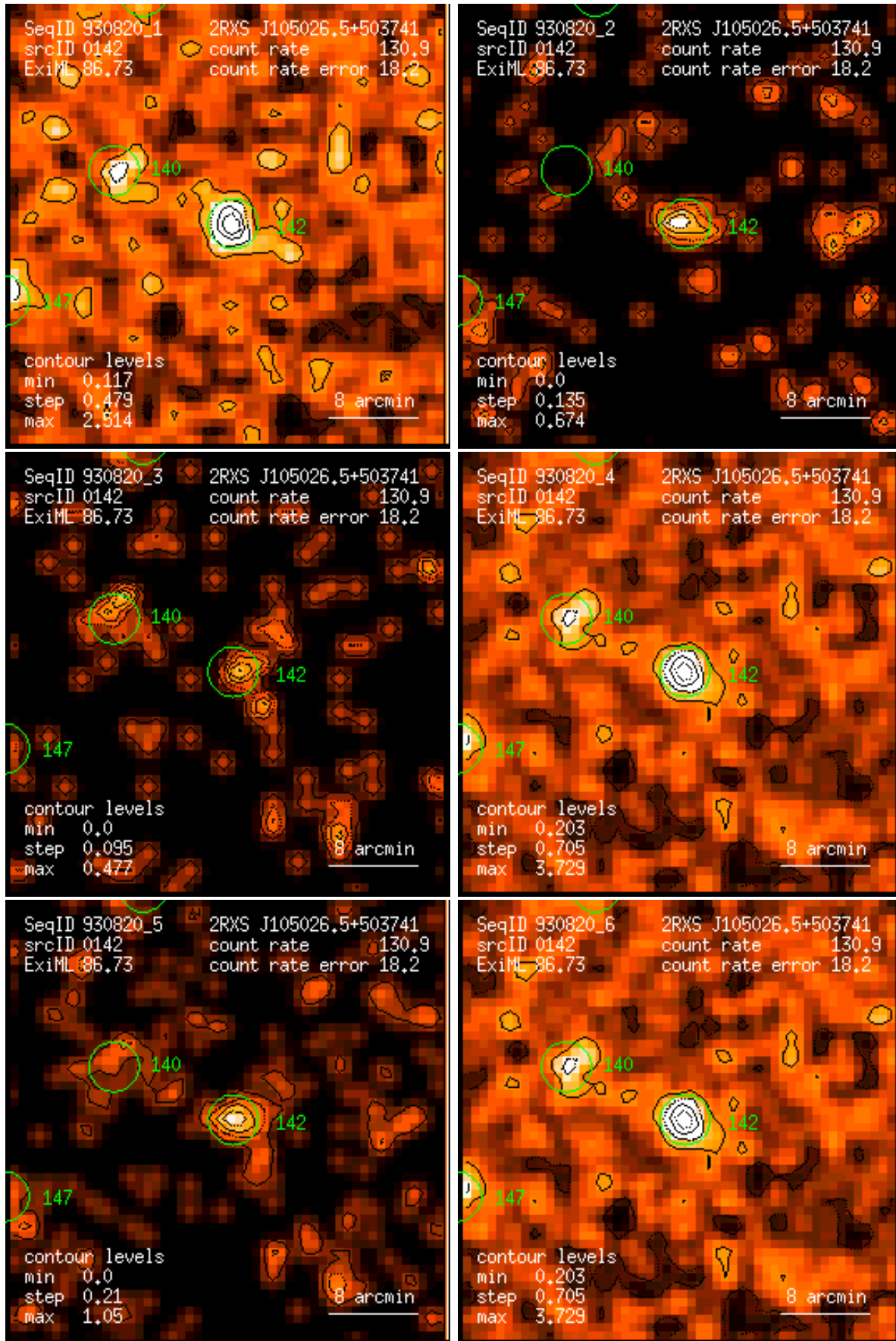
Figure 142: RASS 930820: detection 0142: band rate images, Gaussian filter: (1) PSPC channels 11 – 41, (2) 52 – 90, (3) 91 – 201, (4) 11 – 235, (5) 52 – 201, (6) 11 – 201. Broad band rates in counts/ks. Band rate contour levels in counts/ks/arcmin 2 .
