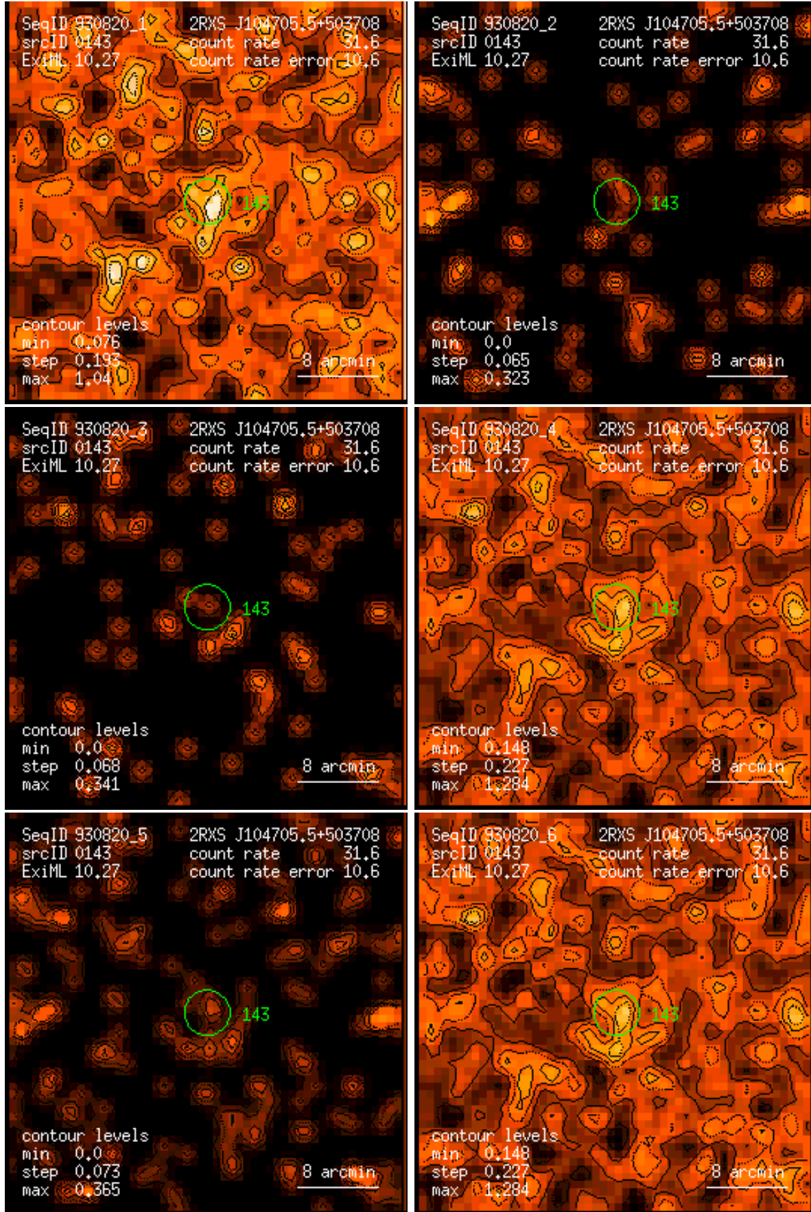
Figure 143: RASS 930820: detection 0143: band rate images, Gaussian filter: (1) PSPC channels 11 – 41, (2) 52 – 90, (3) 91 – 201, (4) 11 – 235, (5) 52 – 201, (6) 11 – 201. Broad band rates in counts/ks. Band rate contour levels in counts/ks/arcmin 2 .
