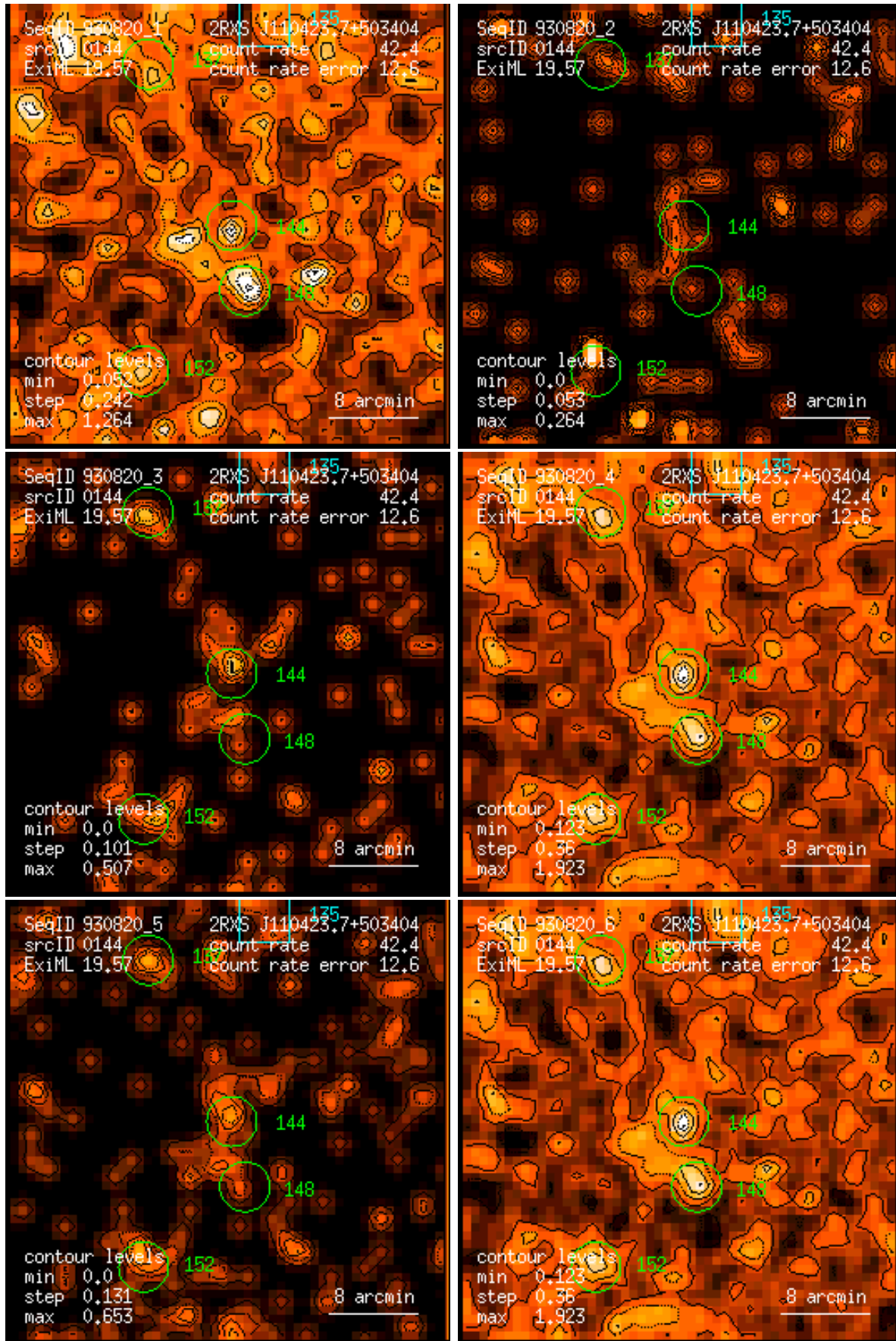
Figure 144: RASS 930820: detection 0144: band rate images, Gaussian filter: (1) PSPC channels 11 – 41, (2) 52 – 90, (3) 91 – 201, (4) 11 – 235, (5) 52 – 201, (6) 11 – 201. Broad band rates in counts/ks. Band rate contour levels in counts/ks/arcmin 2 .
