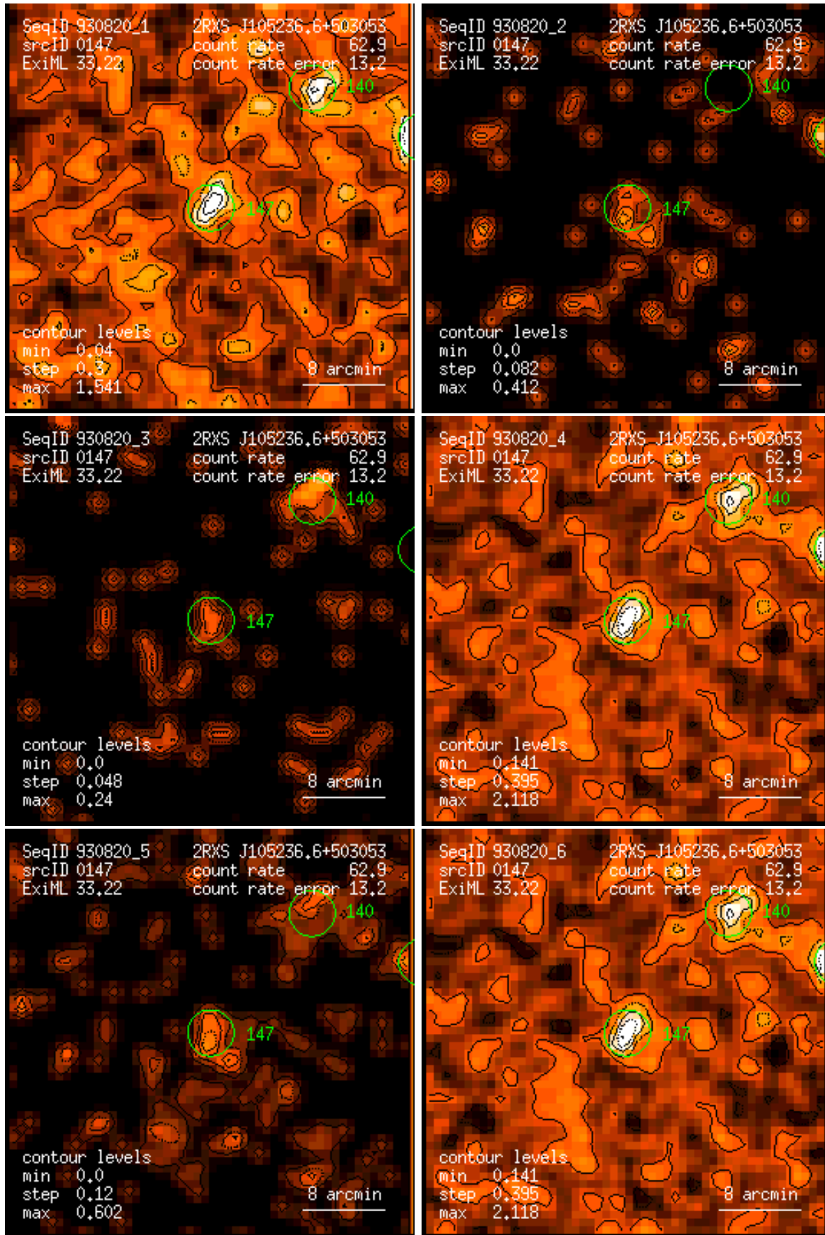
Figure 147: RASS 930820: detection 0147: band rate images, Gaussian filter: (1) PSPC channels 11 – 41, (2) 52 – 90, (3) 91 – 201, (4) 11 – 235, (5) 52 – 201, (6) 11 – 201. Broad band rates in counts/ks. Band rate contour levels in counts/ks/arcmin 2 .
