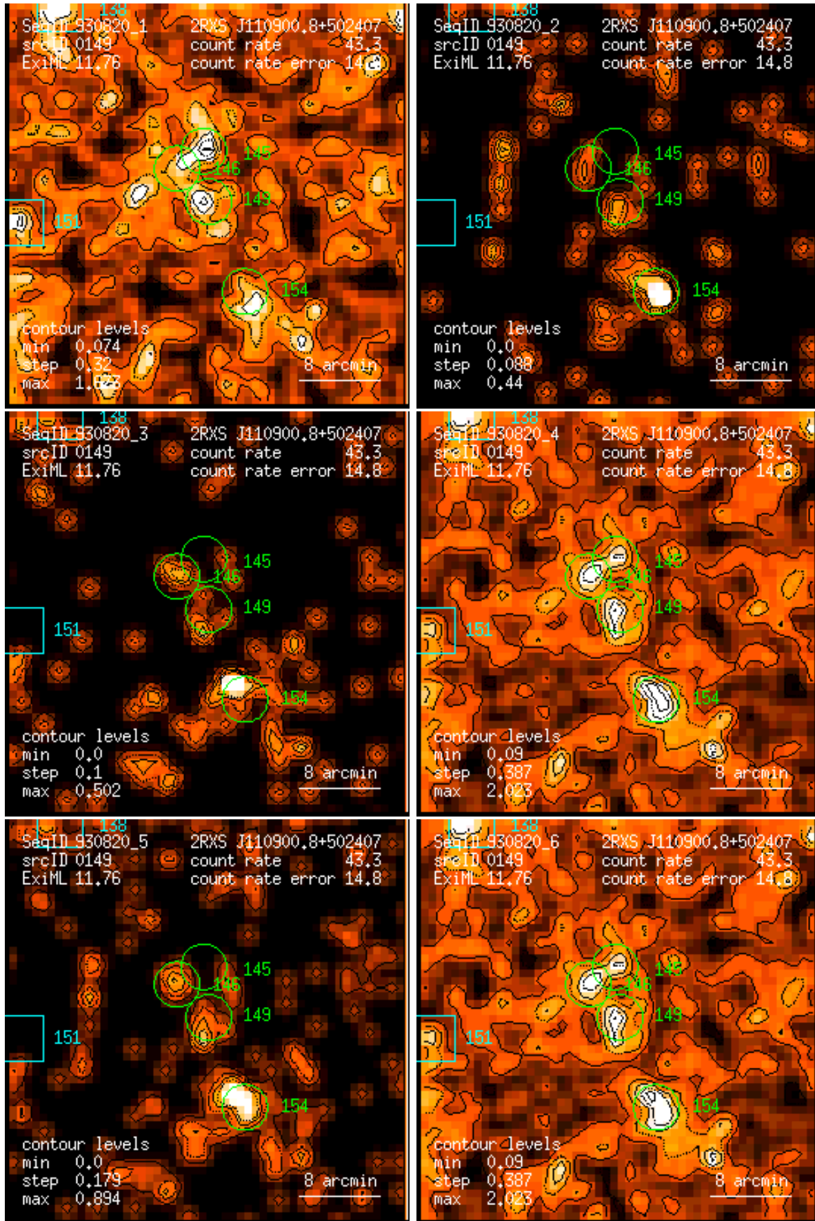
Figure 149: RASS 930820: detection 0149: band rate images, Gaussian filter: (1) PSPC channels 11 – 41, (2) 52 – 90, (3) 91 – 201, (4) 11 – 235, (5) 52 – 201, (6) 11 – 201. Broad band rates in counts/ks. Band rate contour levels in counts/ks/arcmin 2 .
