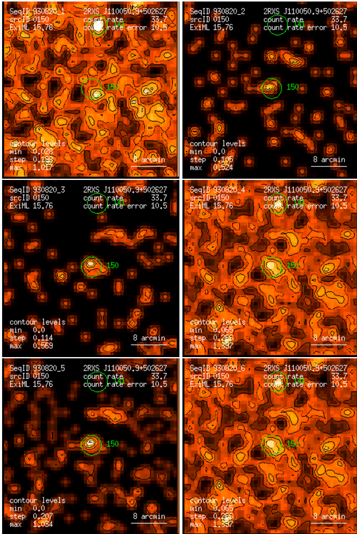
Figure 150: RASS 930820: detection 0150: band rate images, Gaussian filter: (1) PSPC channels 11 – 41, (2) 52 – 90, (3) 91 – 201, (4) 11 – 235, (5) 52 – 201, (6) 11 – 201. Broad band rates in counts/ks. Band rate contour levels in counts/ks/arcmin 2 .
