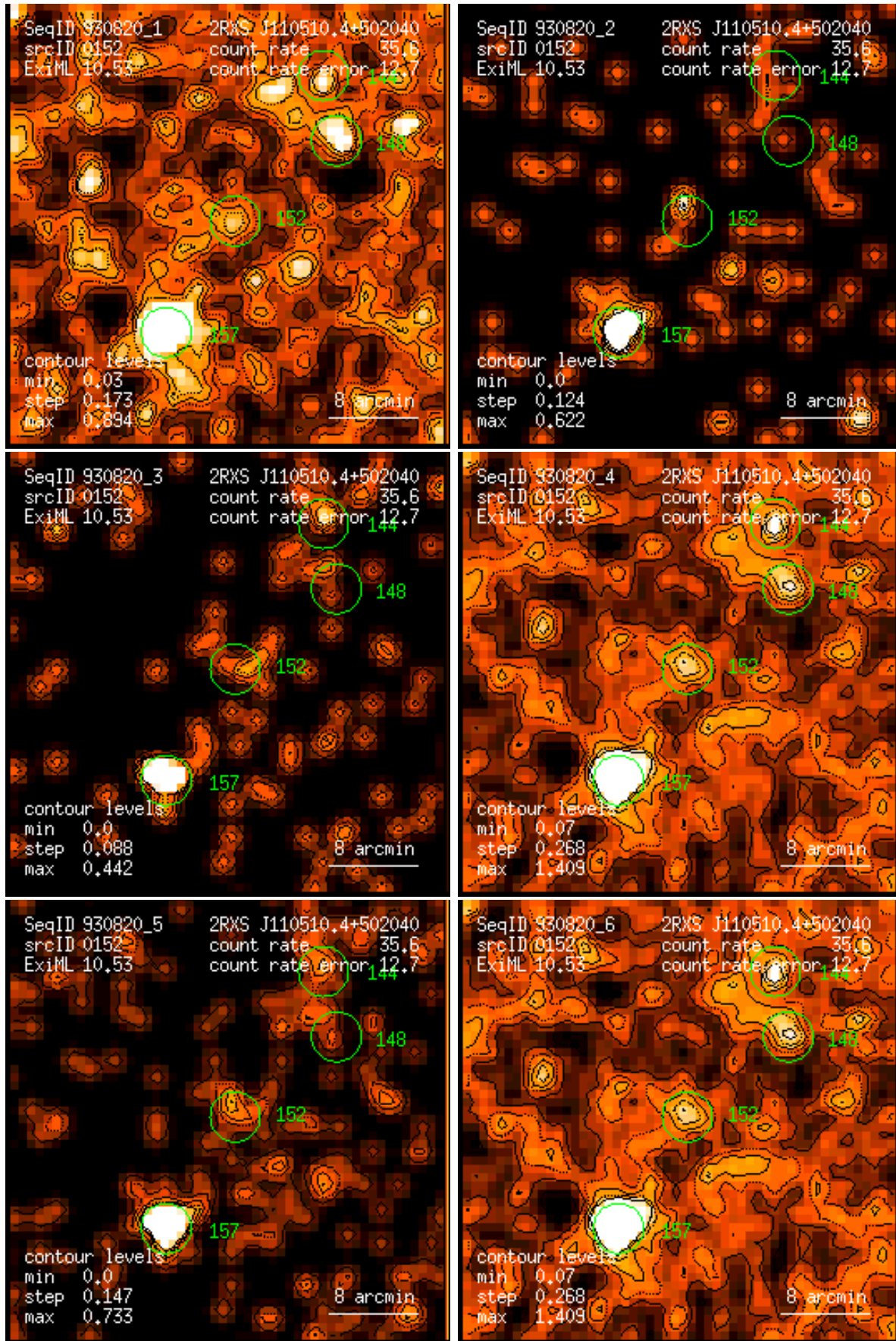
Figure 152: RASS 930820: detection 0152: band rate images, Gaussian filter: (1) PSPC channels 11 – 41, (2) 52 – 90, (3) 91 – 201, (4) 11 – 235, (5) 52 – 201, (6) 11 – 201. Broad band rates in counts/ks. Band rate contour levels in counts/ks/arcmin 2 .
