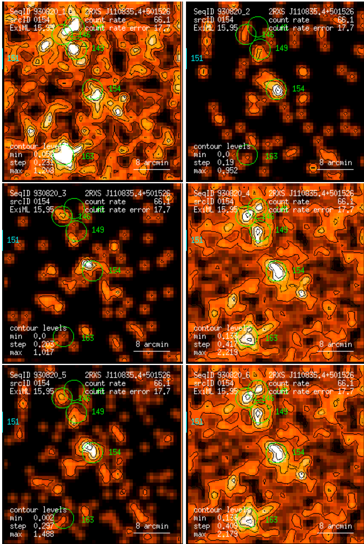
Figure 154: RASS 930820: detection 0154: band rate images, Gaussian filter: (1) PSPC channels 11 – 41, (2) 52 – 90, (3) 91 – 201, (4) 11 – 235, (5) 52 – 201, (6) 11 – 201. Broad band rates in counts/ks. Band rate contour levels in counts/ks/arcmin 2 .
