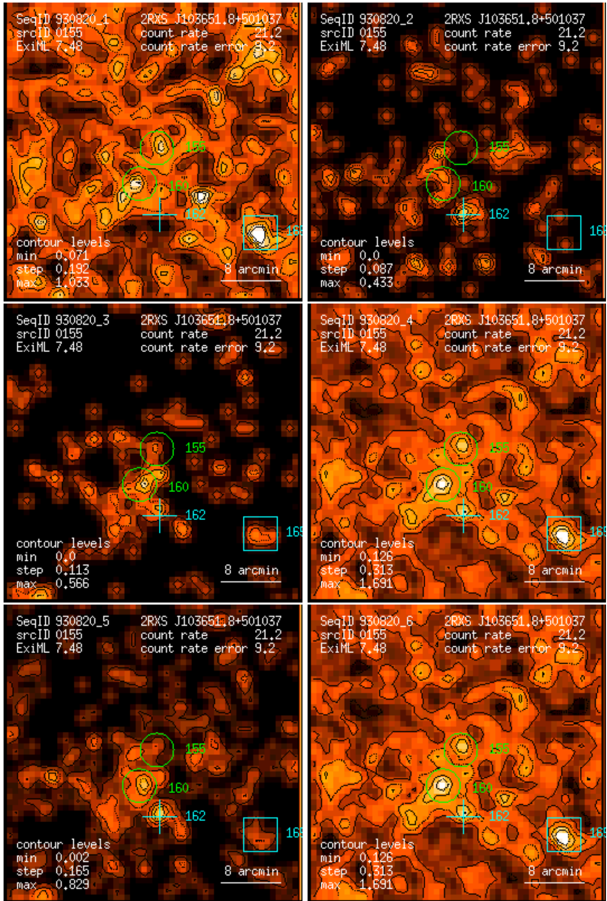
Figure 155: RASS 930820: detection 0155: band rate images, Gaussian filter: (1) PSPC channels 11 – 41, (2) 52 – 90, (3) 91 – 201, (4) 11 – 235, (5) 52 – 201, (6) 11 – 201. Broad band rates in counts/ks. Band rate contour levels in counts/ks/arcmin 2 .
