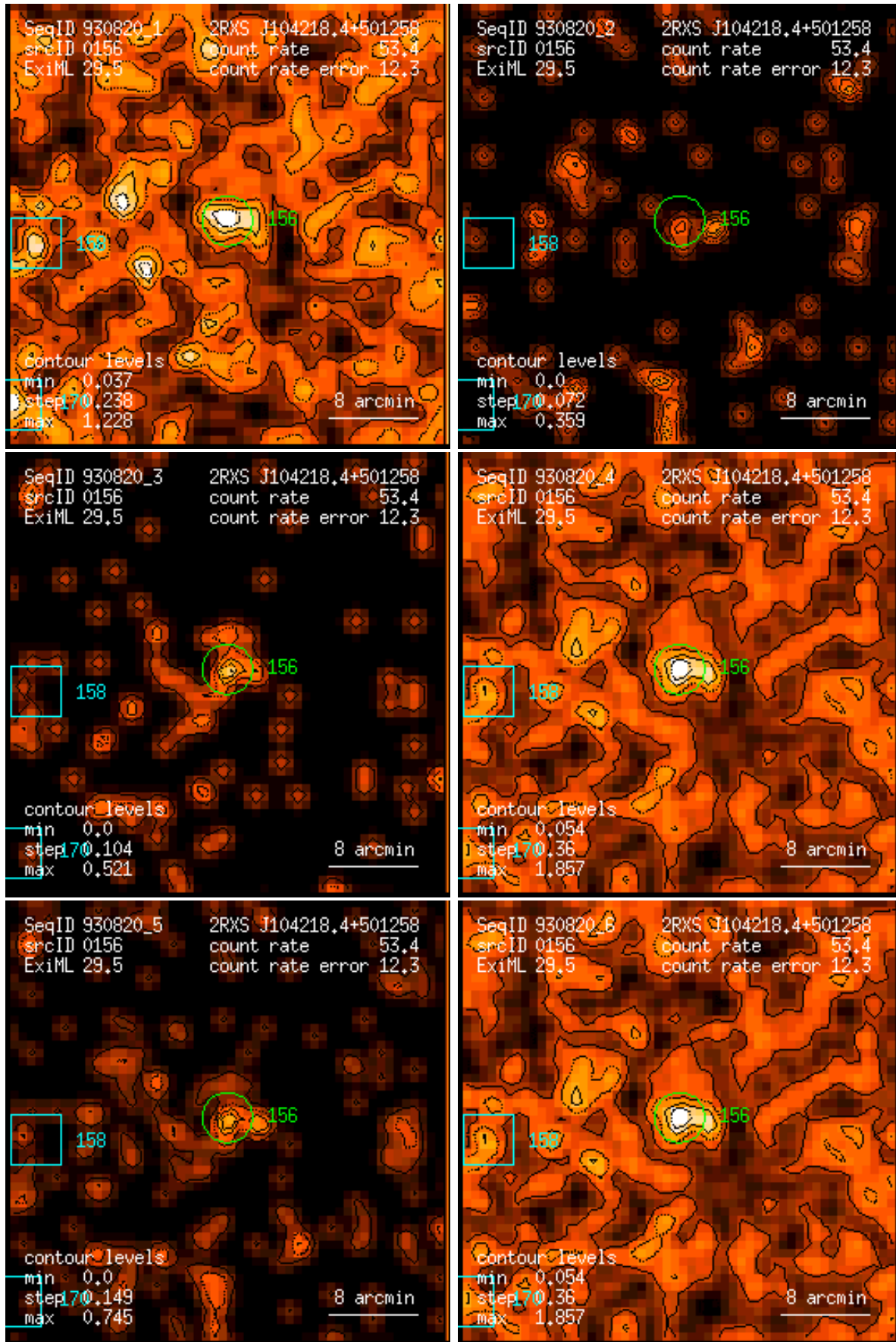
Figure 156: RASS 930820: detection 0156: band rate images, Gaussian filter: (1) PSPC channels 11 – 41, (2) 52 – 90, (3) 91 – 201, (4) 11 – 235, (5) 52 – 201, (6) 11 – 201. Broad band rates in counts/ks. Band rate contour levels in counts/ks/arcmin 2 .
