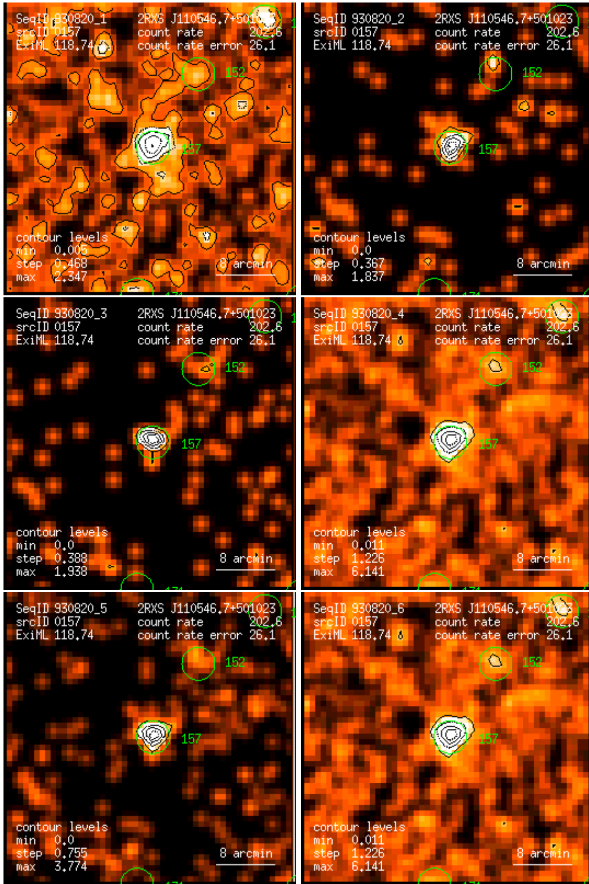
Figure 157: RASS 930820: detection 0157: band rate images, Gaussian filter: (1) PSPC channels 11 – 41, (2) 52 – 90, (3) 91 – 201, (4) 11 – 235, (5) 52 – 201, (6) 11 – 201. Broad band rates in counts/ks. Band rate contour levels in counts/ks/arcmin 2 .
