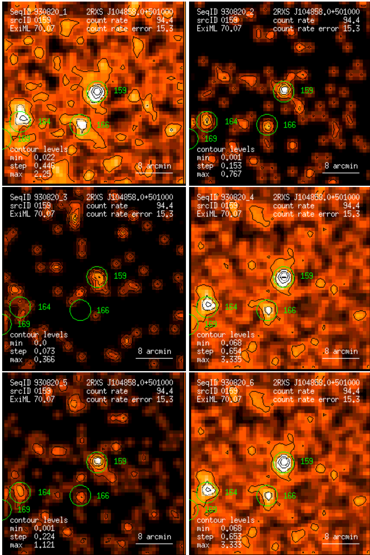
Figure 159: RASS 930820: detection 0159: band rate images, Gaussian filter: (1) PSPC channels 11 – 41, (2) 52 – 90, (3) 91 – 201, (4) 11 – 235, (5) 52 – 201, (6) 11 – 201. Broad band rates in counts/ks. Band rate contour levels in counts/ks/arcmin 2 .
