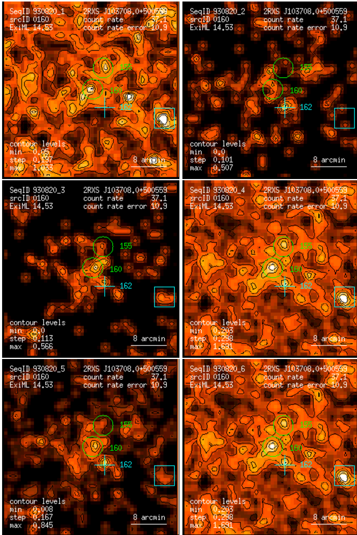
Figure 160: RASS 930820: detection 0160: band rate images, Gaussian filter: (1) PSPC channels 11 – 41, (2) 52 – 90, (3) 91 – 201, (4) 11 – 235, (5) 52 – 201, (6) 11 – 201. Broad band rates in counts/ks. Band rate contour levels in counts/ks/arcmin 2 .
