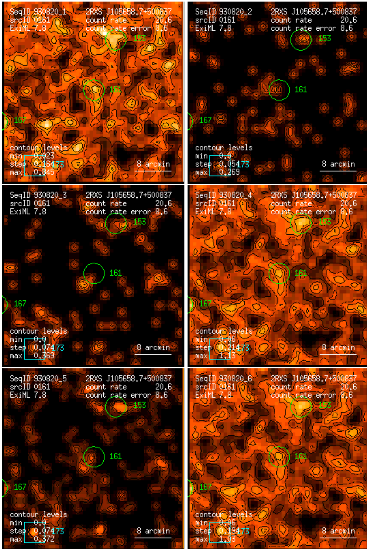
Figure 161: RASS 930820: detection 0161: band rate images, Gaussian filter: (1) PSPC channels 11 – 41, (2) 52 – 90, (3) 91 – 201, (4) 11 – 235, (5) 52 – 201, (6) 11 – 201. Broad band rates in counts/ks. Band rate contour levels in counts/ks/arcmin 2 .
