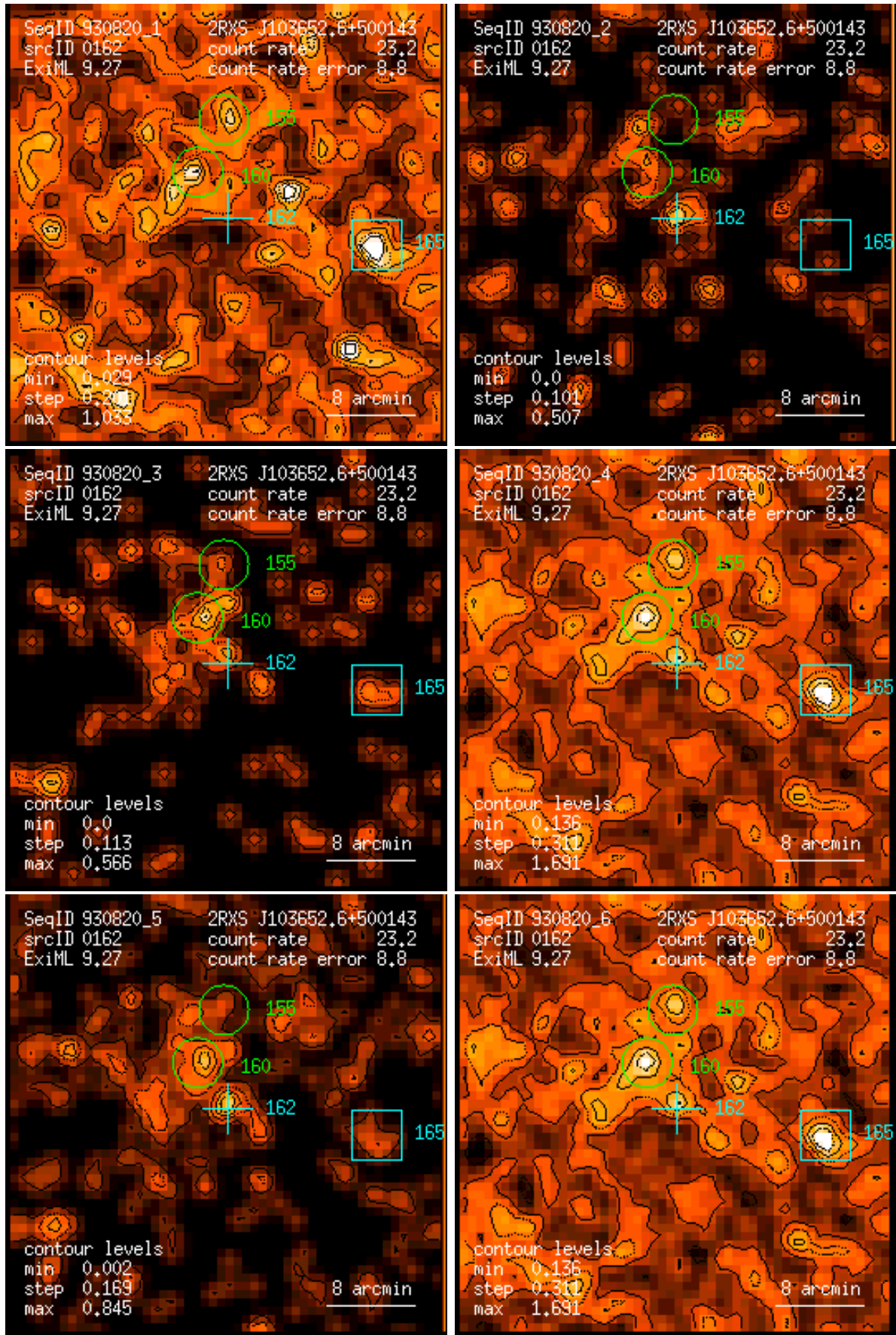
Figure 162: RASS 930820: detection 0162: band rate images, Gaussian filter: (1) PSPC channels 11 – 41, (2) 52 – 90, (3) 91 – 201, (4) 11 – 235, (5) 52 – 201, (6) 11 – 201. Broad band rates in counts/ks. Band rate contour levels in counts/ks/arcmin 2 .
