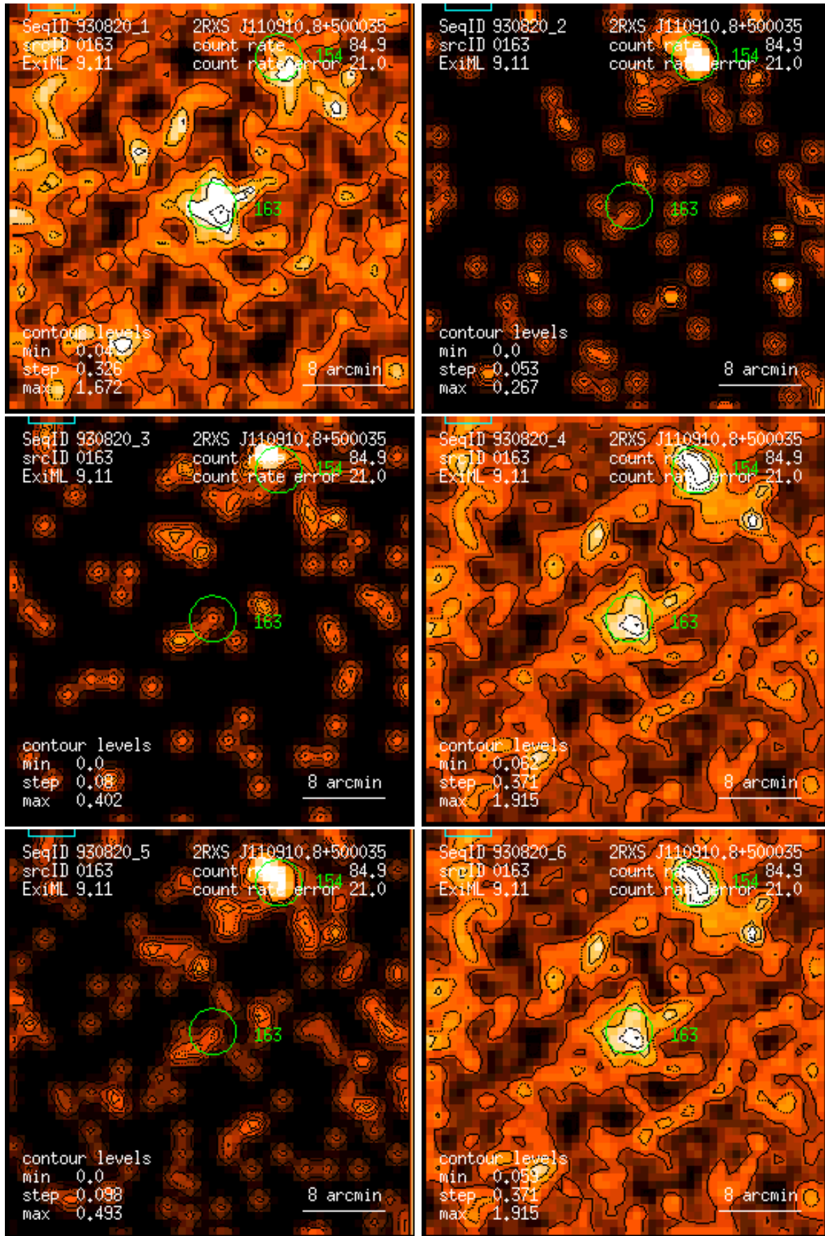
Figure 163: RASS 930820: detection 0163: band rate images, Gaussian filter: (1) PSPC channels 11 – 41, (2) 52 – 90, (3) 91 – 201, (4) 11 – 235, (5) 52 – 201, (6) 11 – 201. Broad band rates in counts/ks. Band rate contour levels in counts/ks/arcmin 2 .
