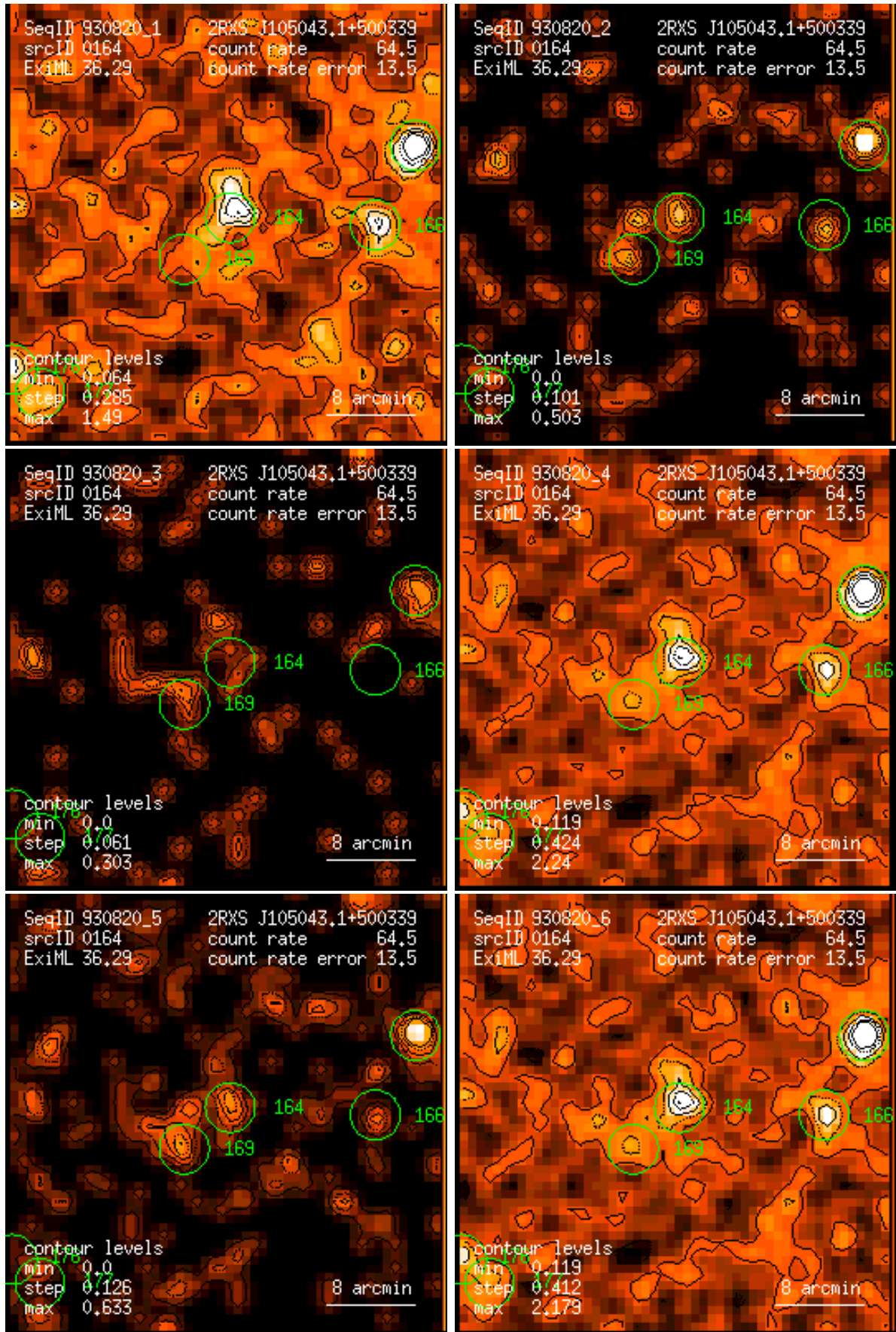
Figure 164: RASS 930820: detection 0164: band rate images, Gaussian filter: (1) PSPC channels 11 – 41, (2) 52 – 90, (3) 91 – 201, (4) 11 – 235, (5) 52 – 201, (6) 11 – 201. Broad band rates in counts/ks. Band rate contour levels in counts/ks/arcmin 2 .
