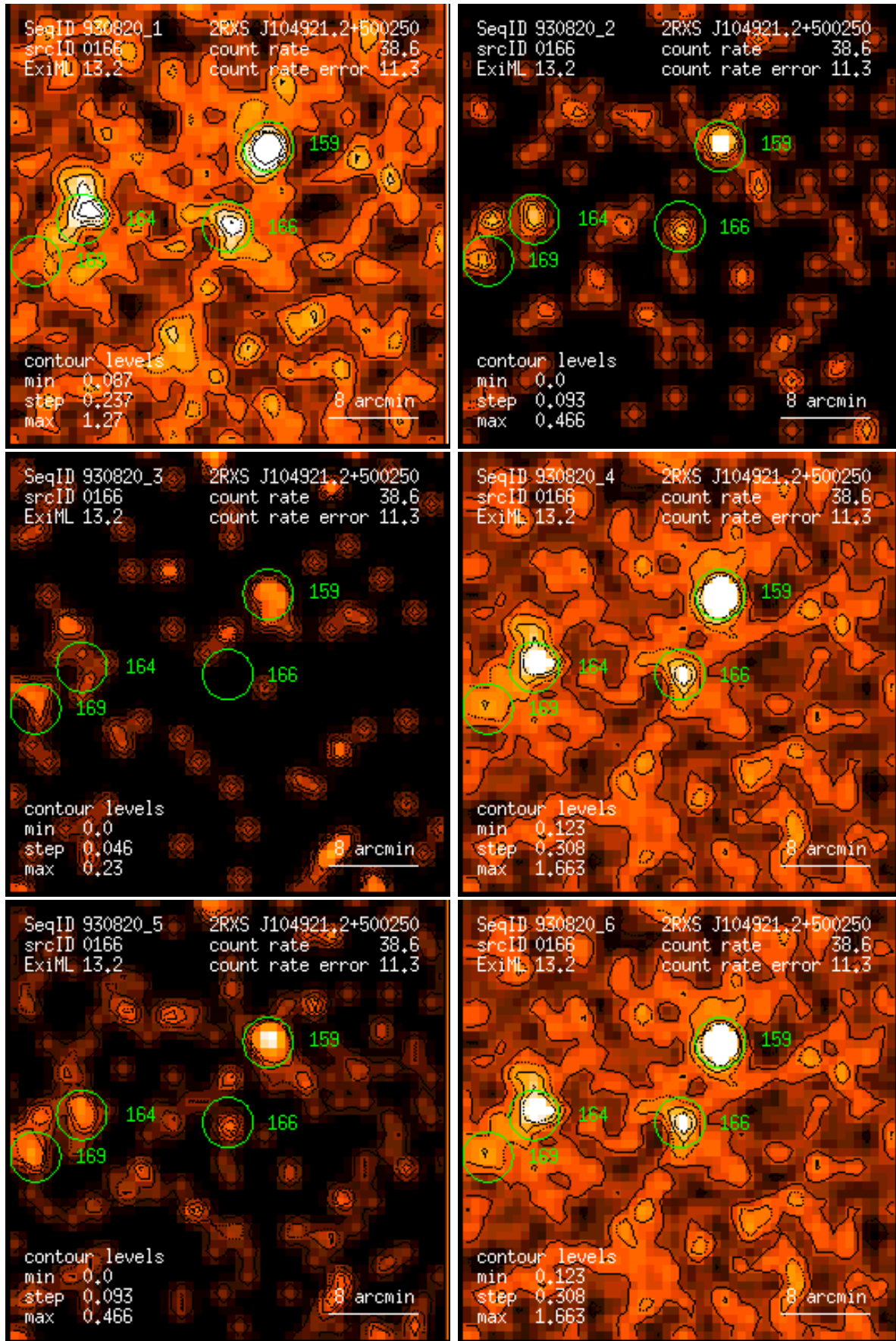
Figure 166: RASS 930820: detection 0166: band rate images, Gaussian filter: (1) PSPC channels 11 – 41, (2) 52 – 90, (3) 91 – 201, (4) 11 – 235, (5) 52 – 201, (6) 11 – 201. Broad band rates in counts/ks. Band rate contour levels in counts/ks/arcmin 2 .
