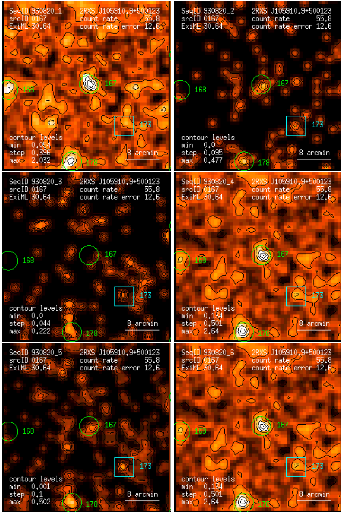
Figure 167: RASS 930820: detection 0167: band rate images, Gaussian filter: (1) PSPC channels 11 – 41, (2) 52 – 90, (3) 91 – 201, (4) 11 – 235, (5) 52 – 201, (6) 11 – 201. Broad band rates in counts/ks. Band rate contour levels in counts/ks/arcmin 2 .
