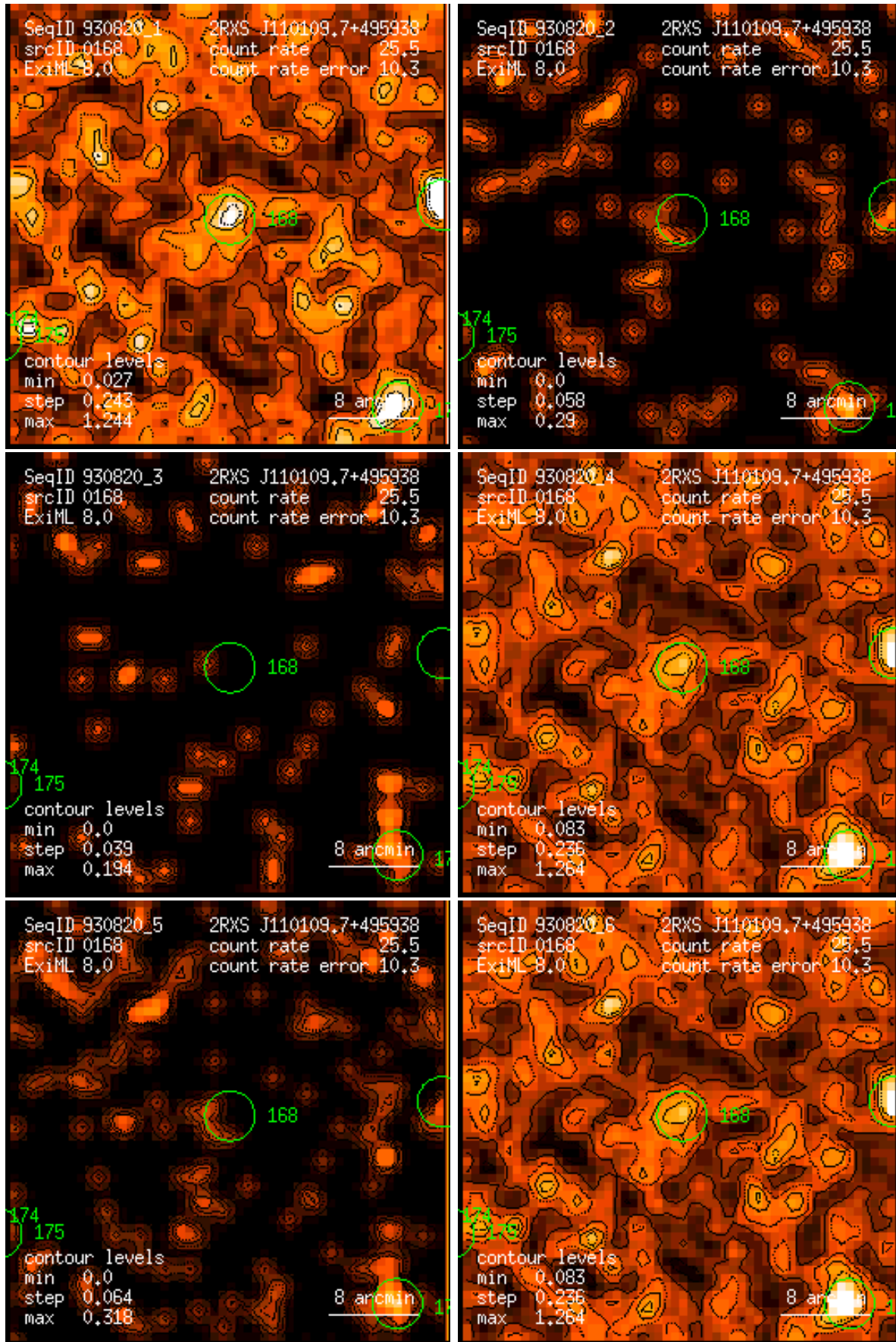
Figure 168: RASS 930820: detection 0168: band rate images, Gaussian filter: (1) PSPC channels 11 – 41, (2) 52 – 90, (3) 91 – 201, (4) 11 – 235, (5) 52 – 201, (6) 11 – 201. Broad band rates in counts/ks. Band rate contour levels in counts/ks/arcmin 2 .
